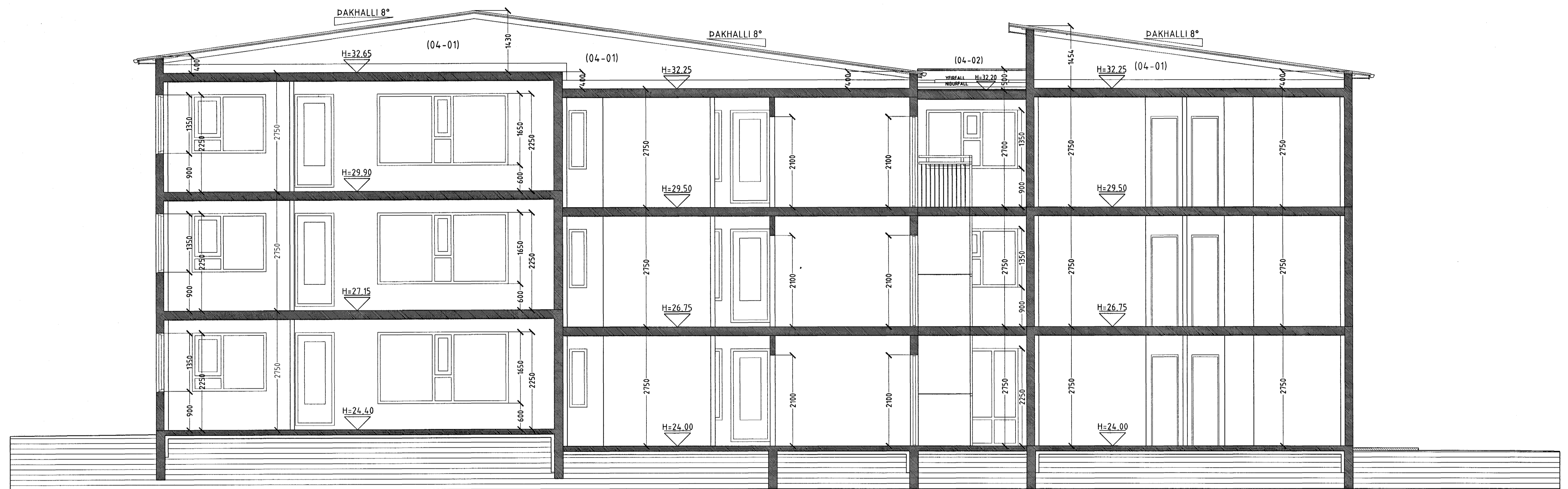
SNID C-C MKV. 1:100.
