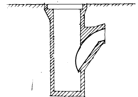
SANDFANG (SF)
