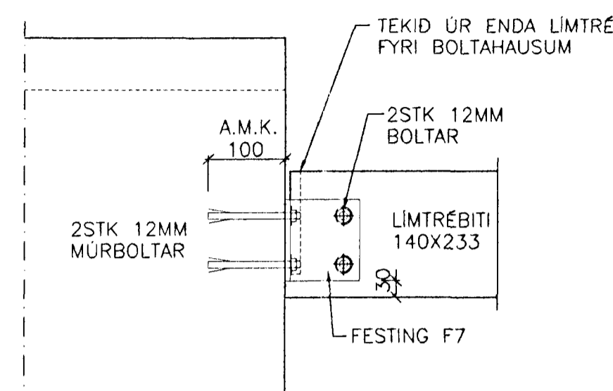
SNID XIa-XIa 1:10
