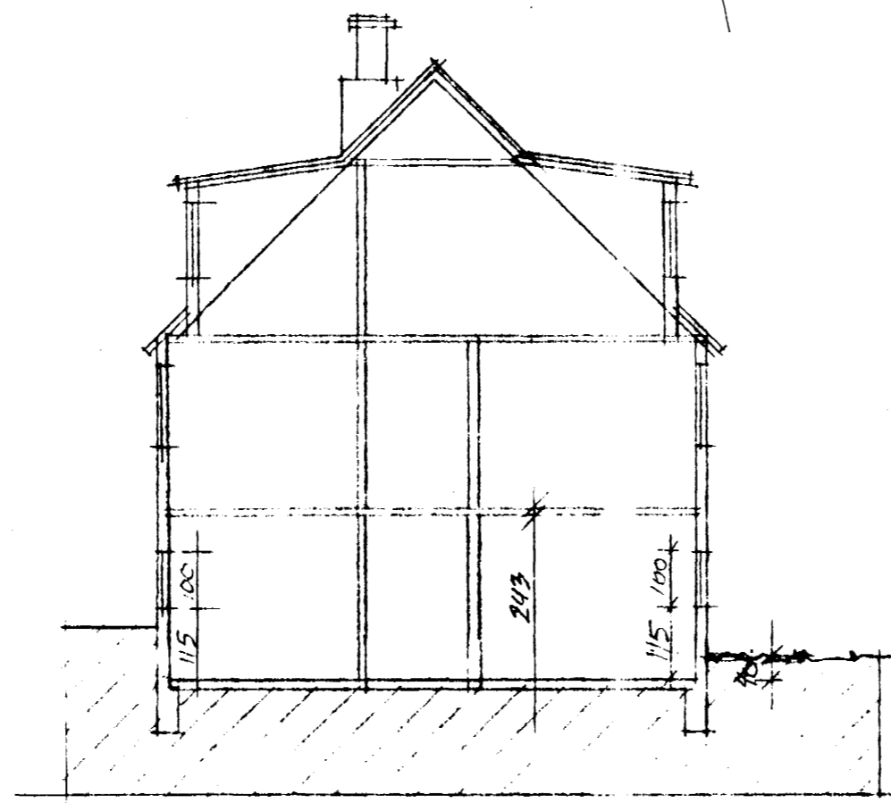
SNIB 1:100
