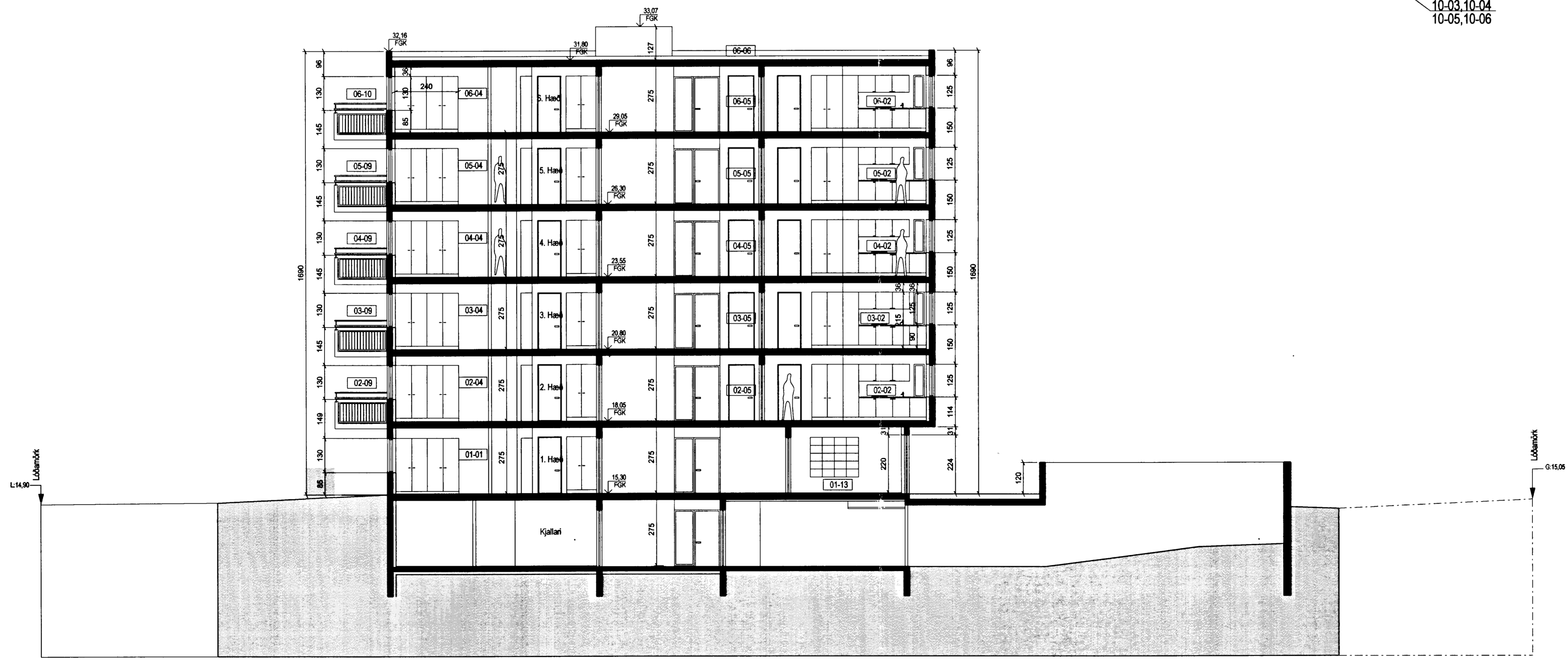
B-B 10-02 SNEIDING 1:100 10-03,10-04 10-05,10-06
