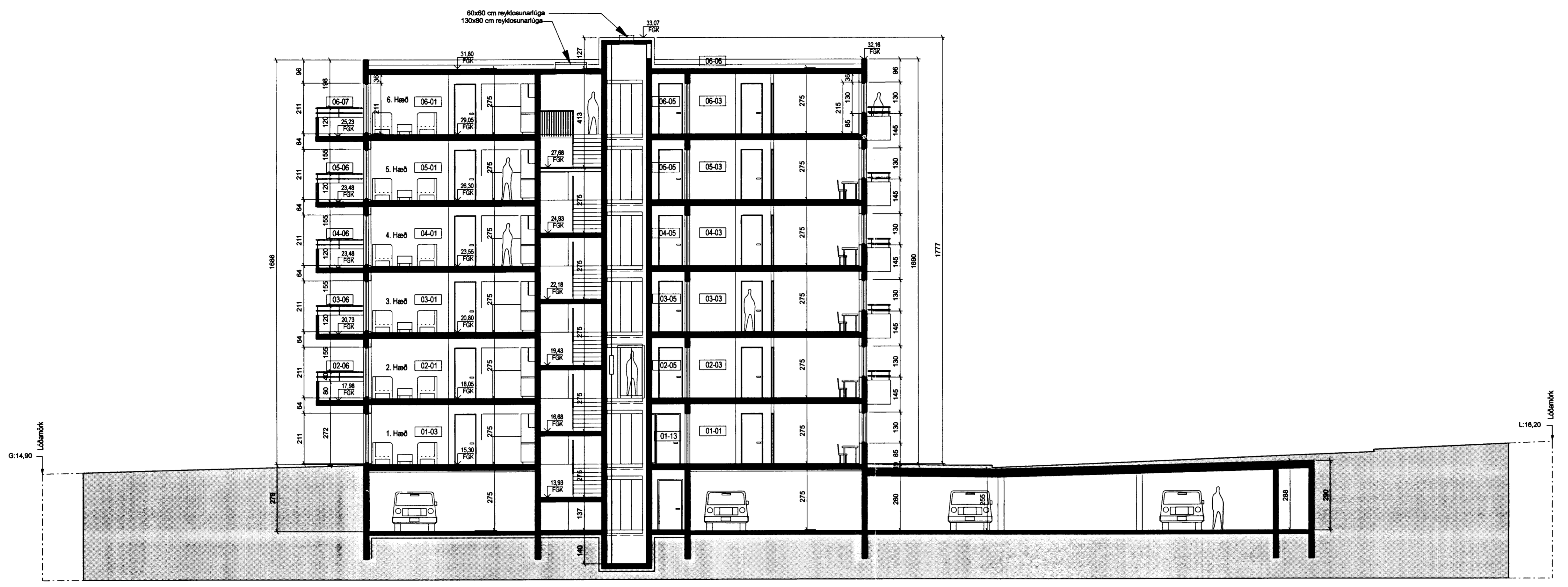
A-A 10-02 SNEIDING 1:100 10-03,10-04 10-05,10-06
