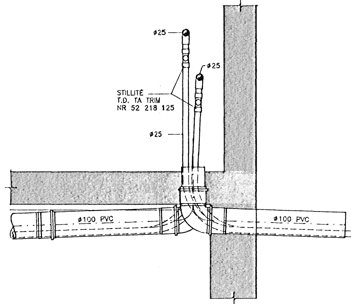
SNJÖBRÆDSLULÖGN. SNID I VEGG. 1:10
