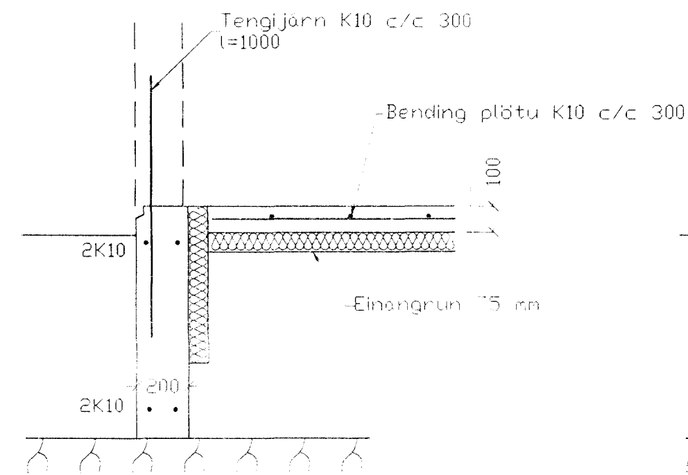
SNID 1, 1:20
