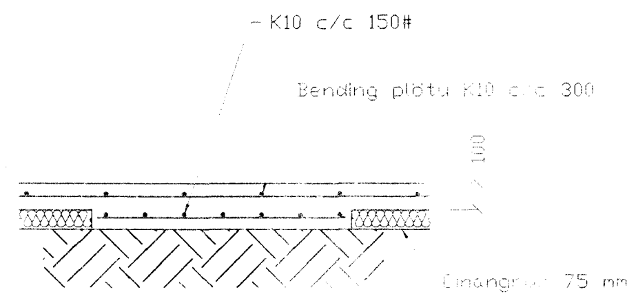
SNID 3, 1:20
