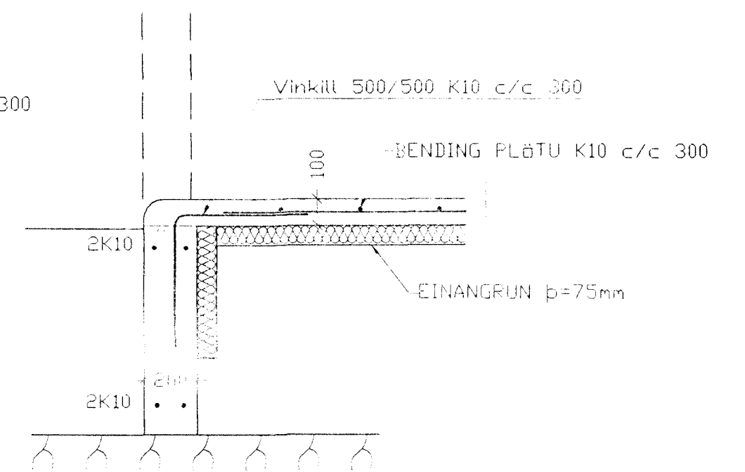
SNID 2, 1:20
