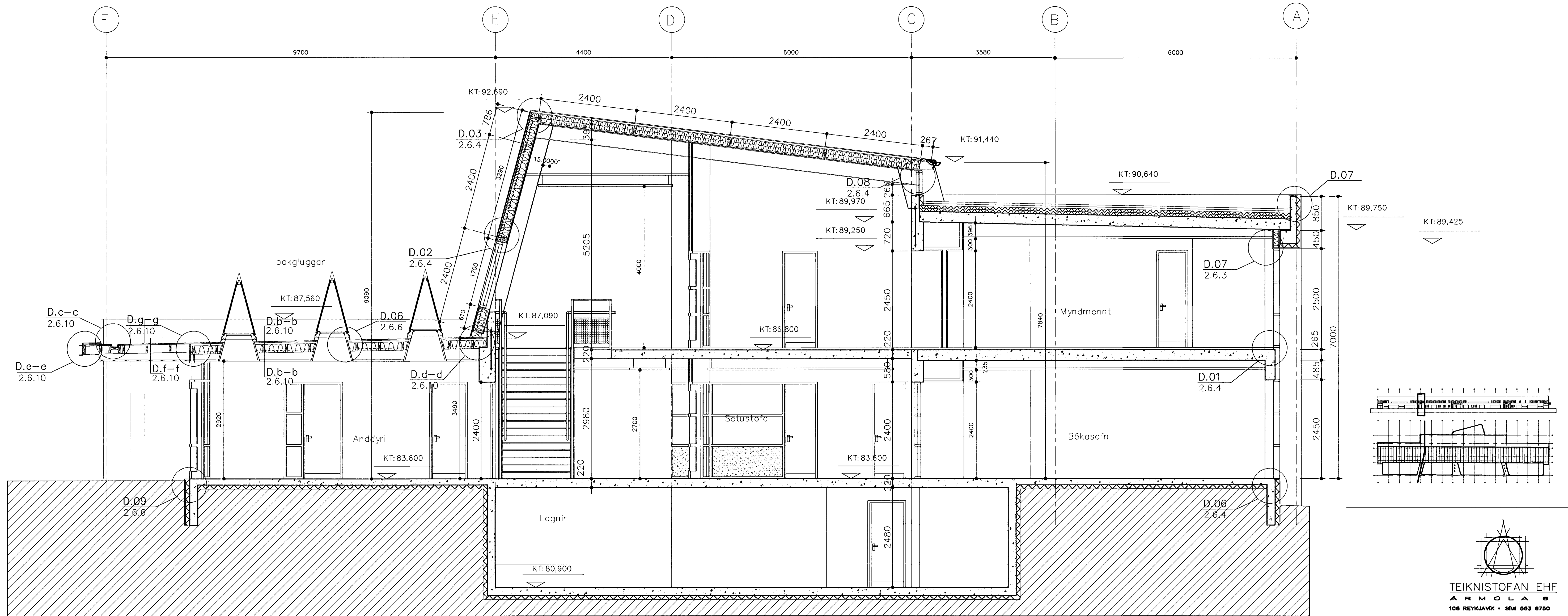
SNEIÐING F-F MKV, 1:50
