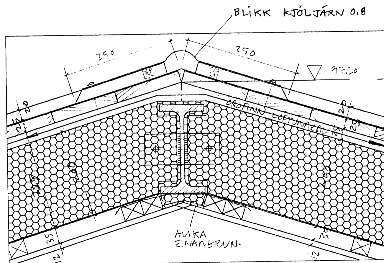
Sneiðing j-j mkv.1:5
