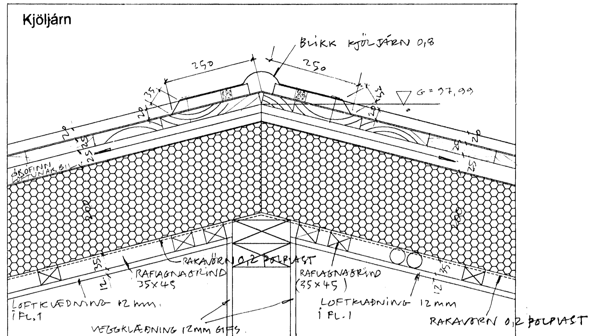
Sneiðing h-h mkv.1:5
