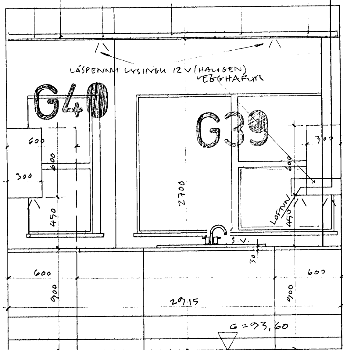
Sneiðing w-w mkv. 1:20
