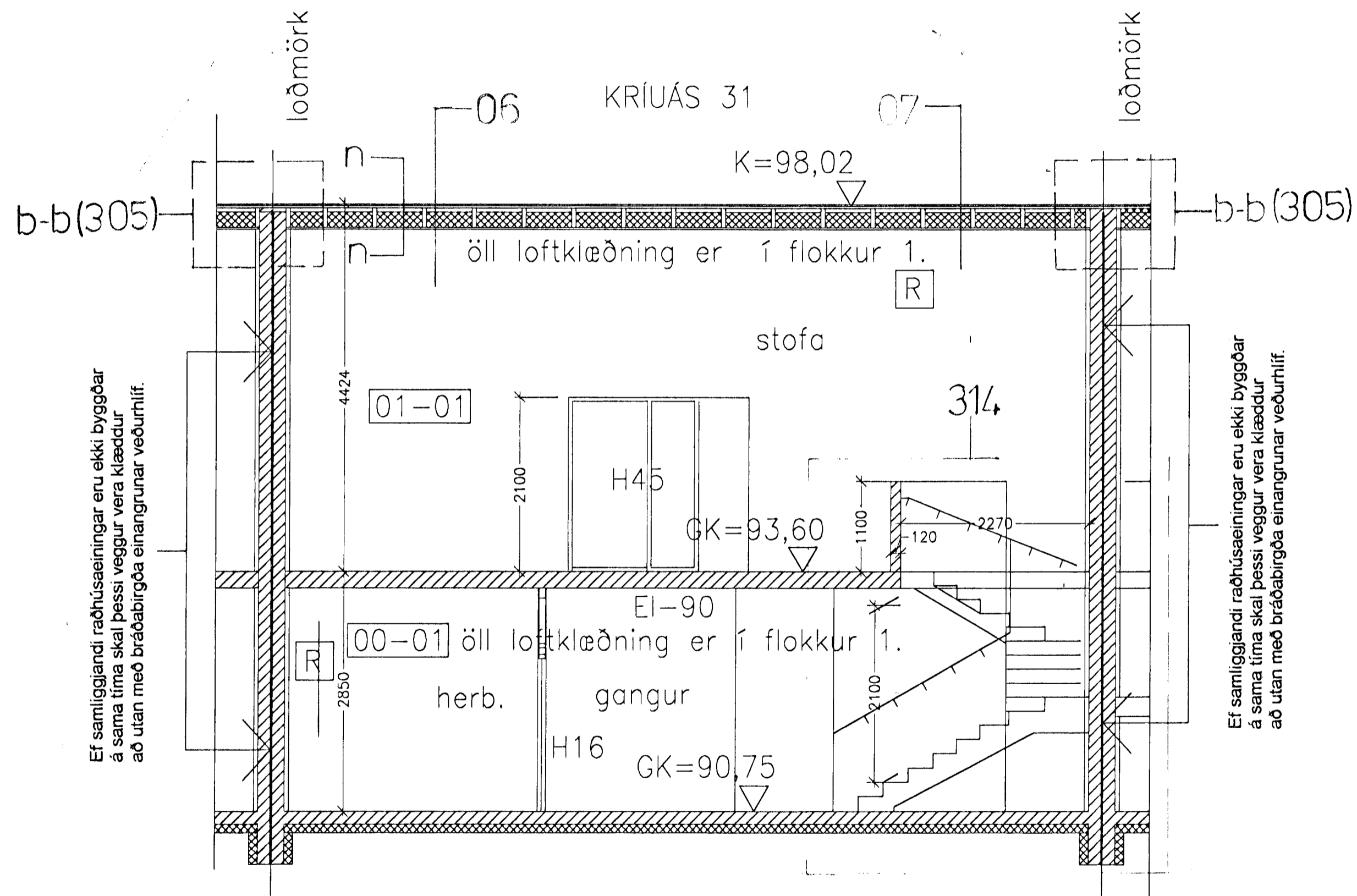
Sneiðing 01-01 mkv.1:50
