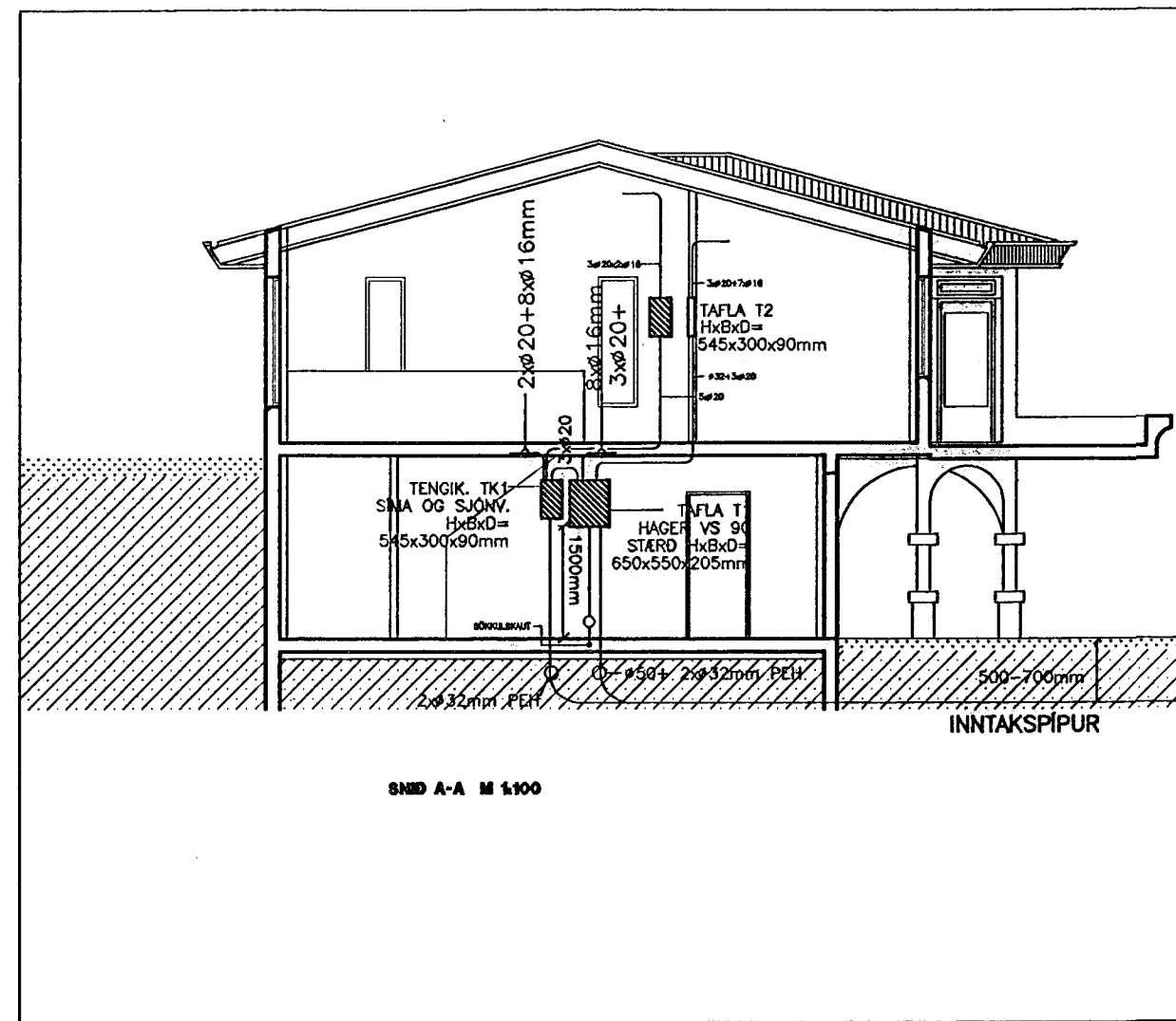
SNID M 1:100
