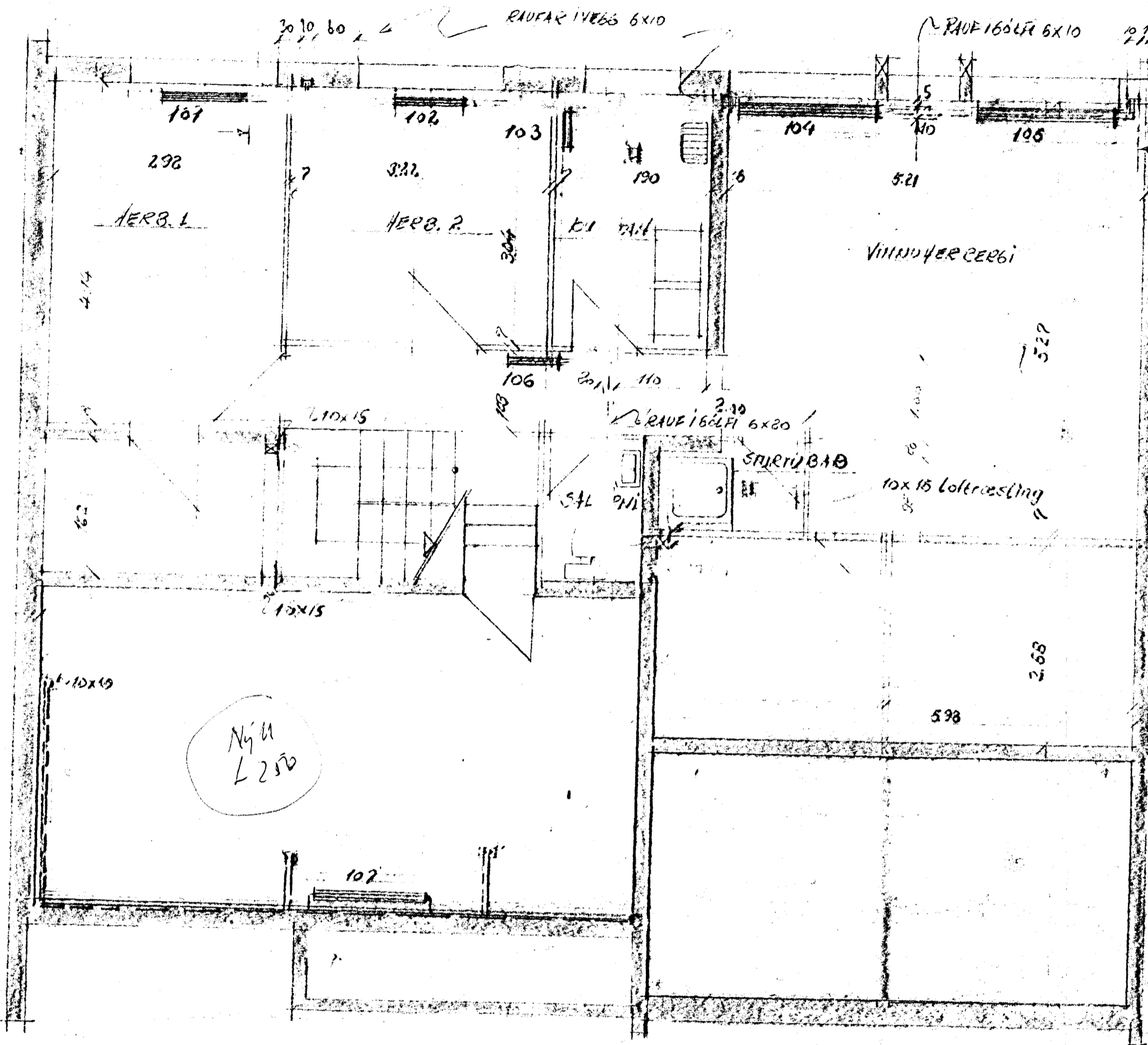
OFNAPLAN Mkv 1:50
