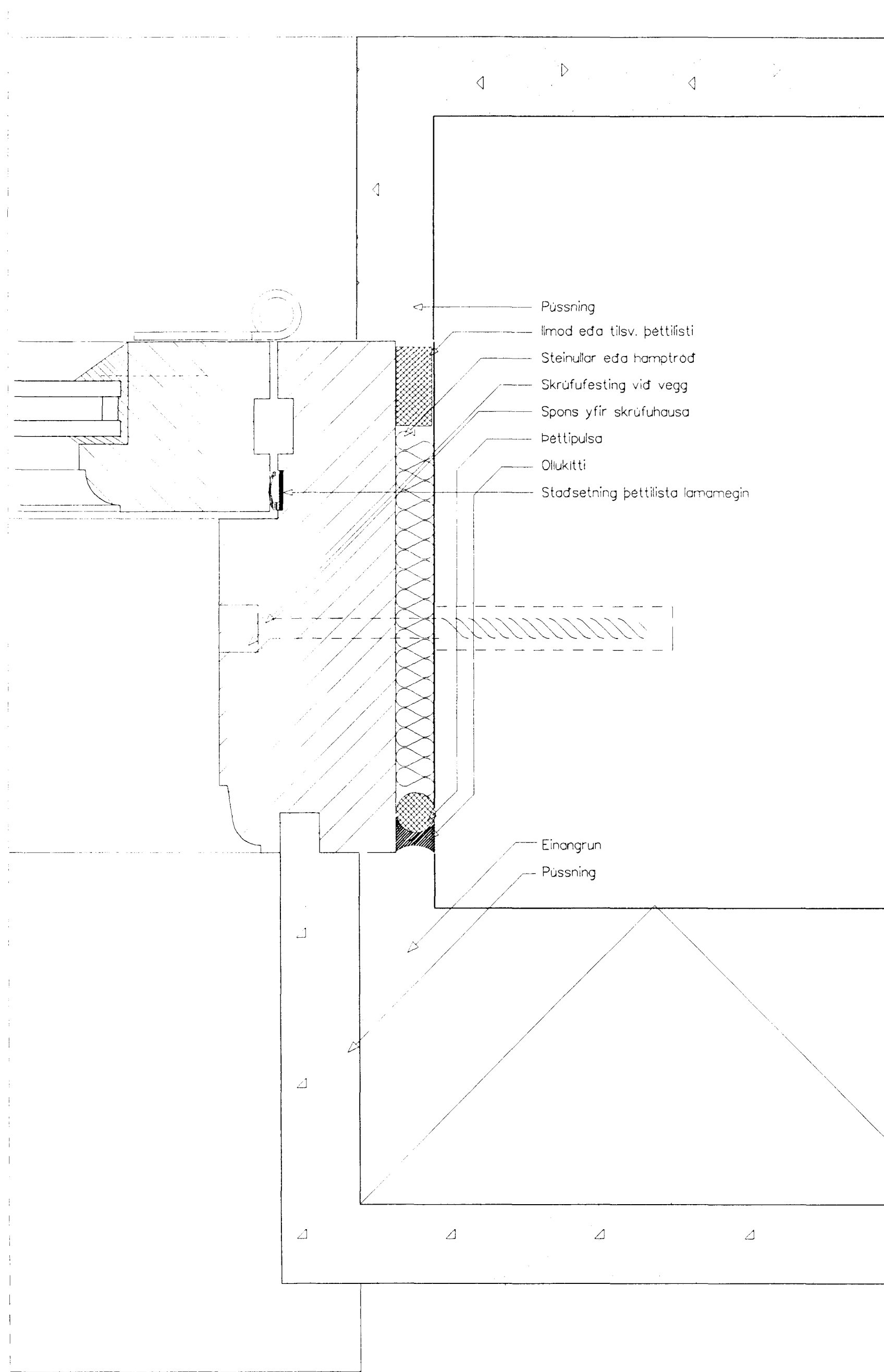
FRAGANGUR GLUGGA I STEINSTEYPTAN VEGG
