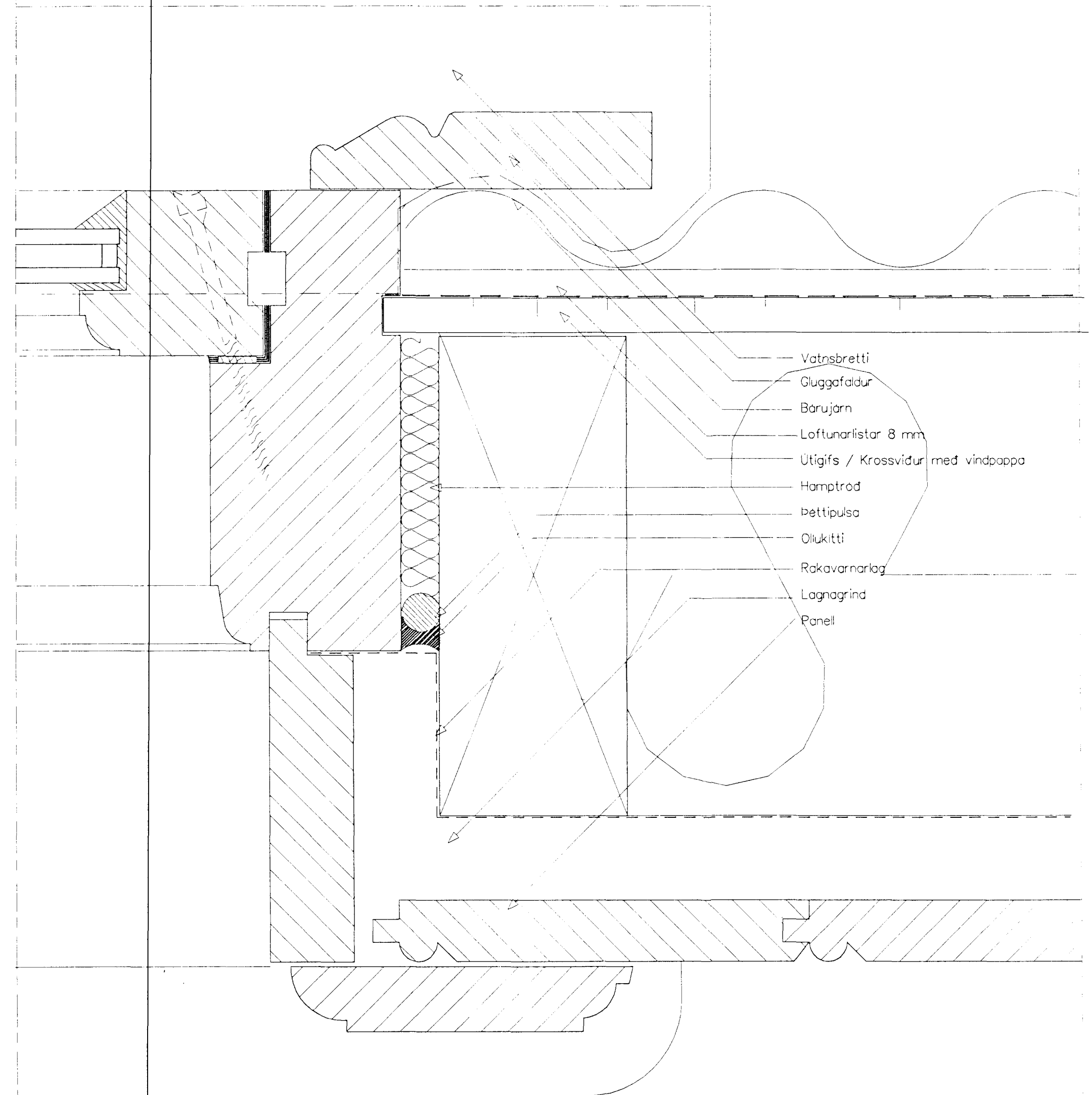
FRAGANGUR GLUGGA I TIMBURVEGG
