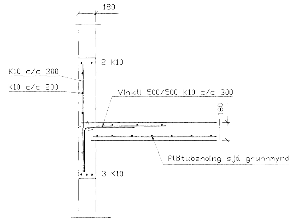
SNID 1, 1:20
