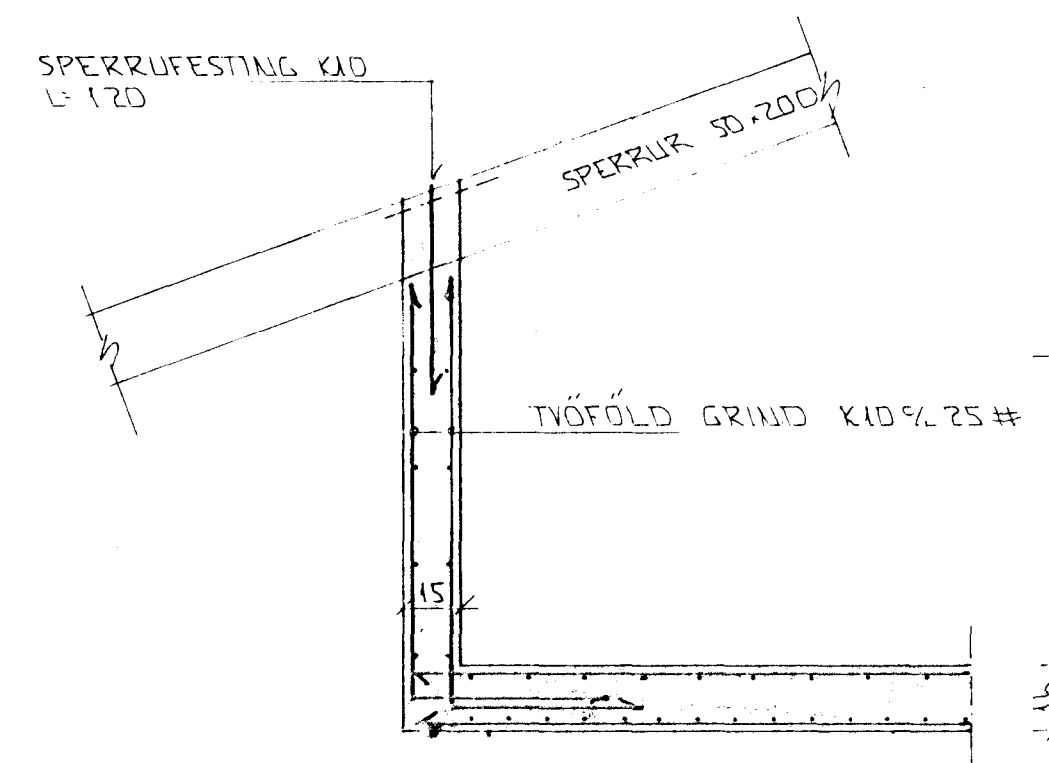
SNIP 11 1:10
