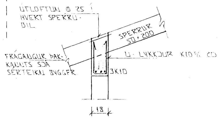
SNIP 13 1:20
