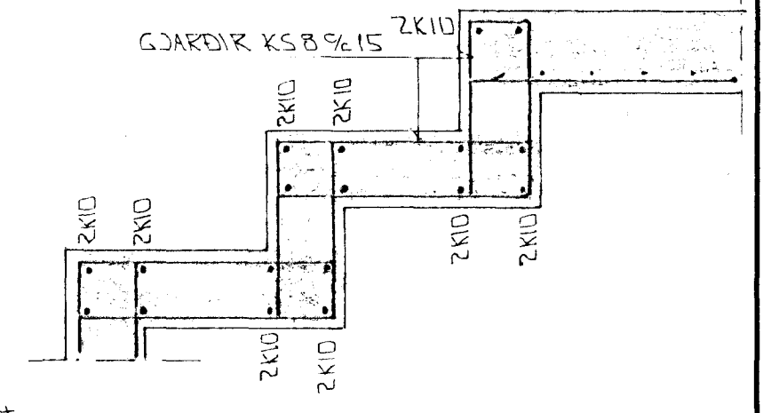
SNIP 11 1:10
