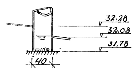
SANDFANG 1:50
