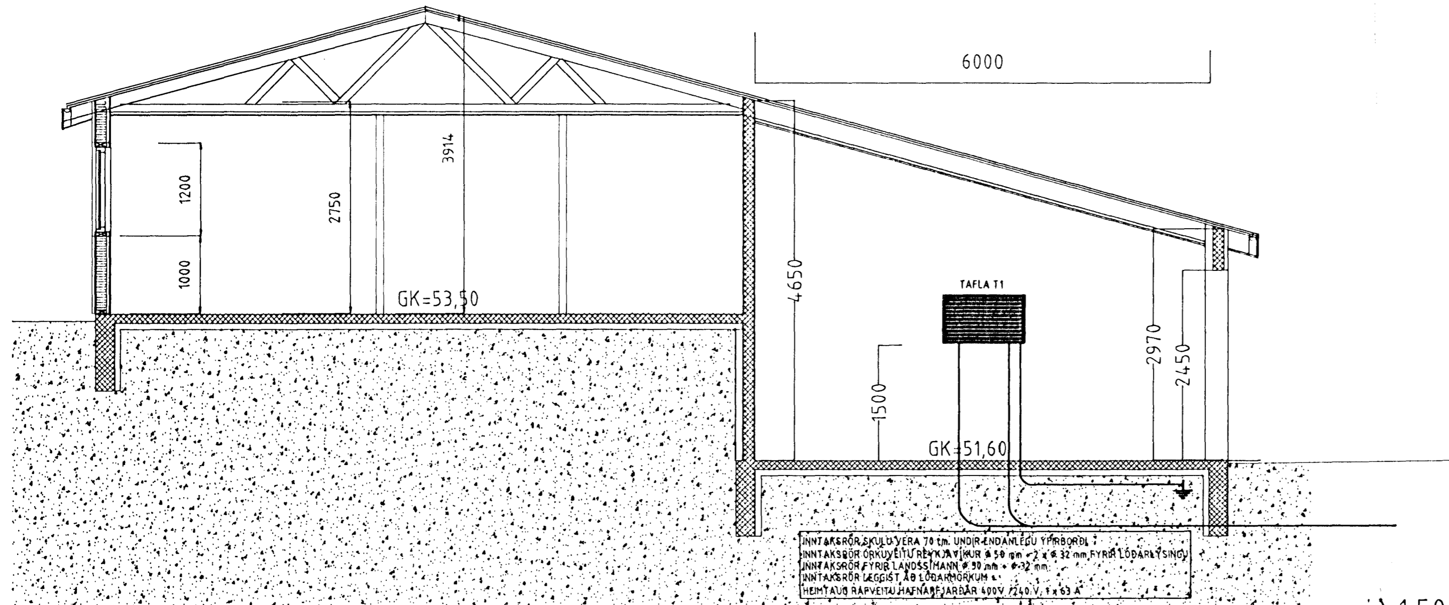
SNID B-B
