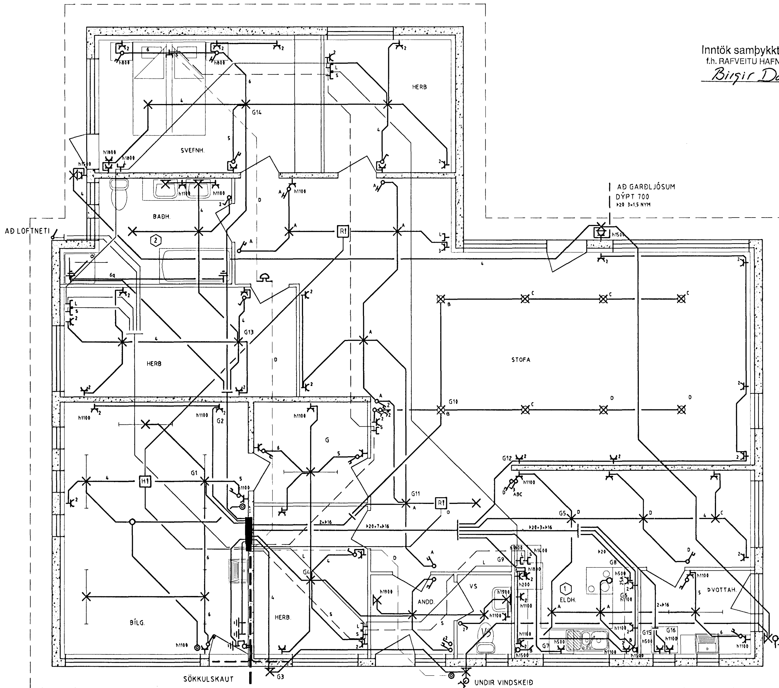
GRUNNPLAN 1:50
