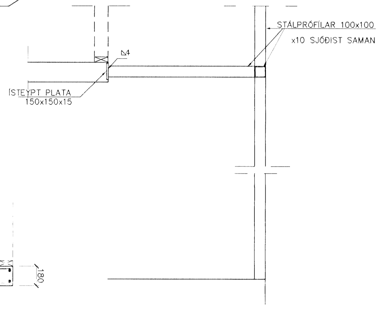
SNID 2-2 1:20
