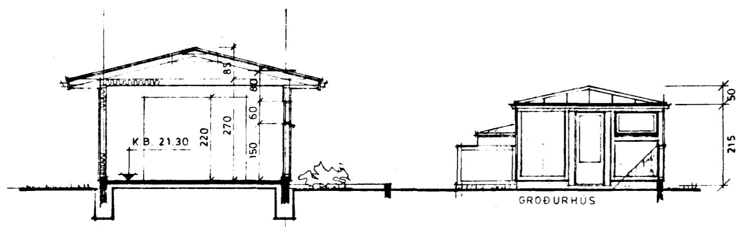
SNID B-B
