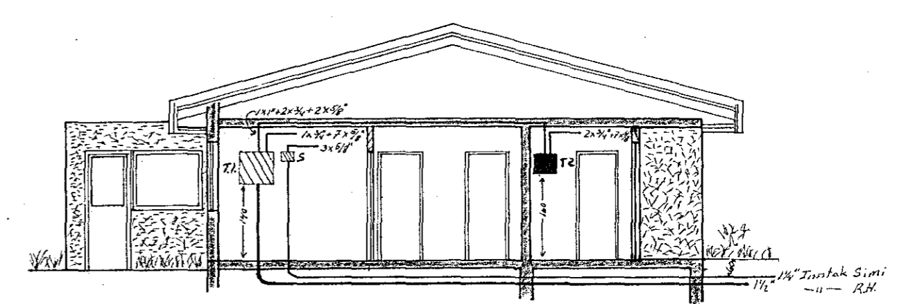
SNID. M: 1:100
