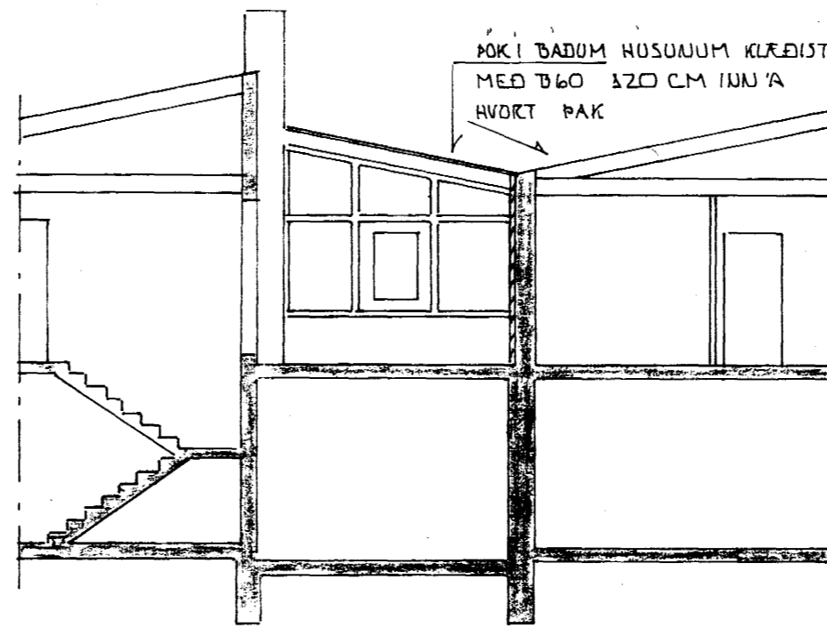
SNID A 1:100
