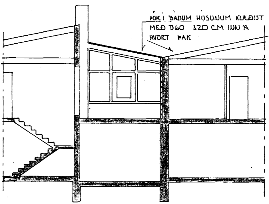
SNID A 1:100
