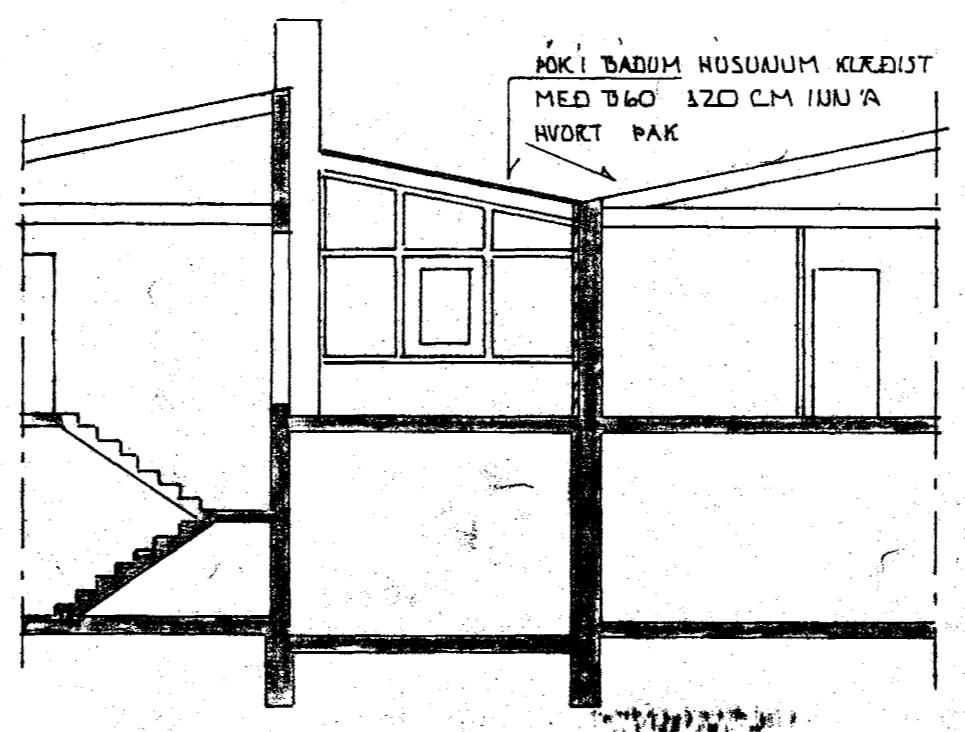
SNID A 1:100
