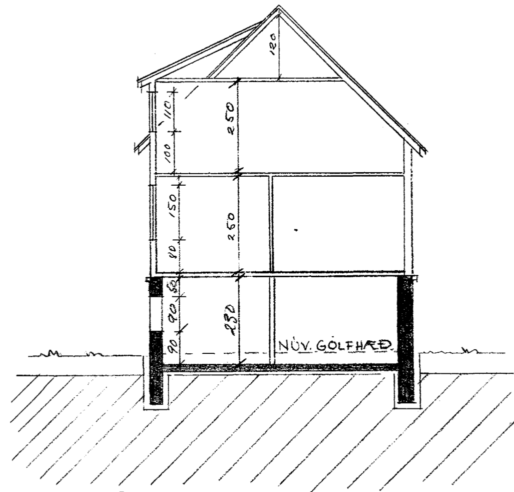
SNID 1:100
