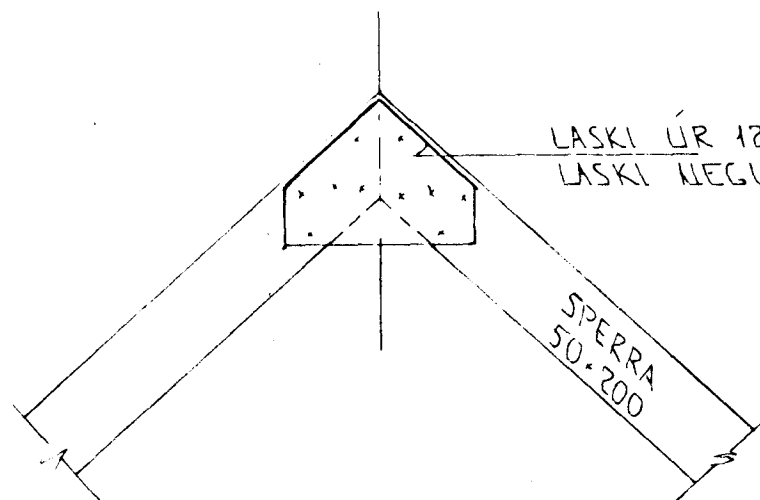
SNID 1-1 1:50
