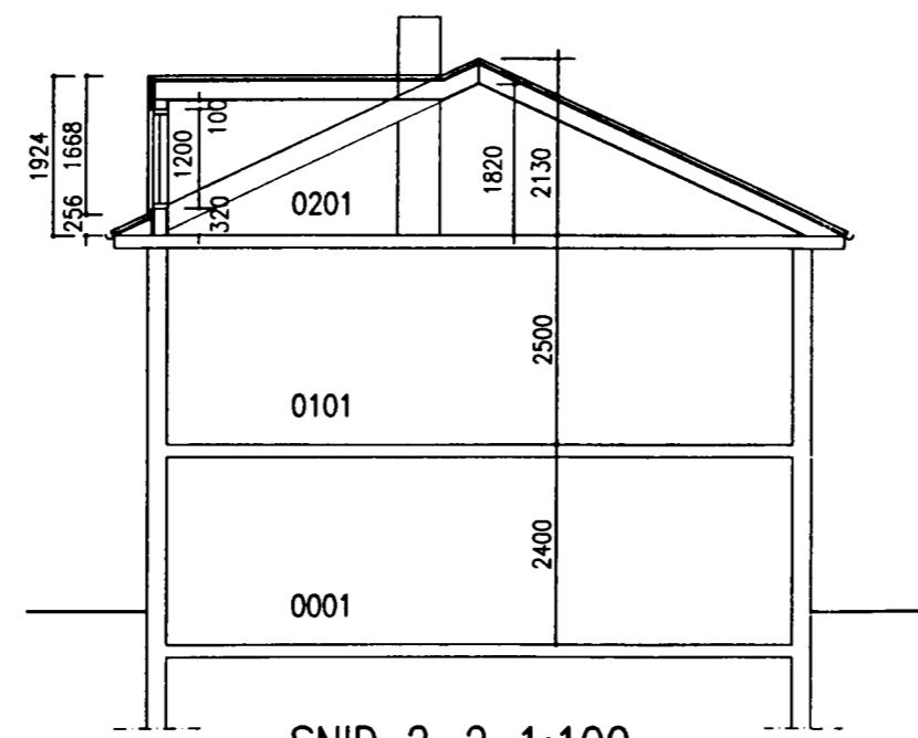
SNID 2-2 1:100
