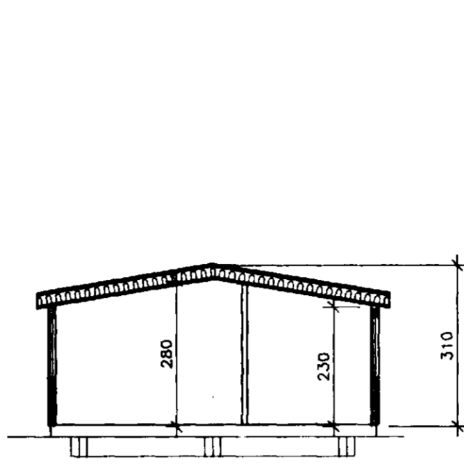
SNID A - A 1:100
