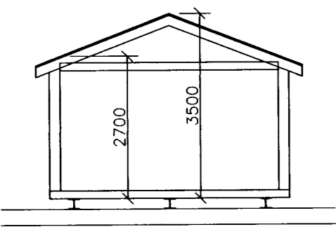
SNID 1:100
