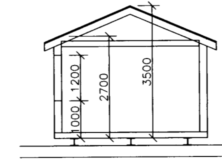
SNID 1:100
