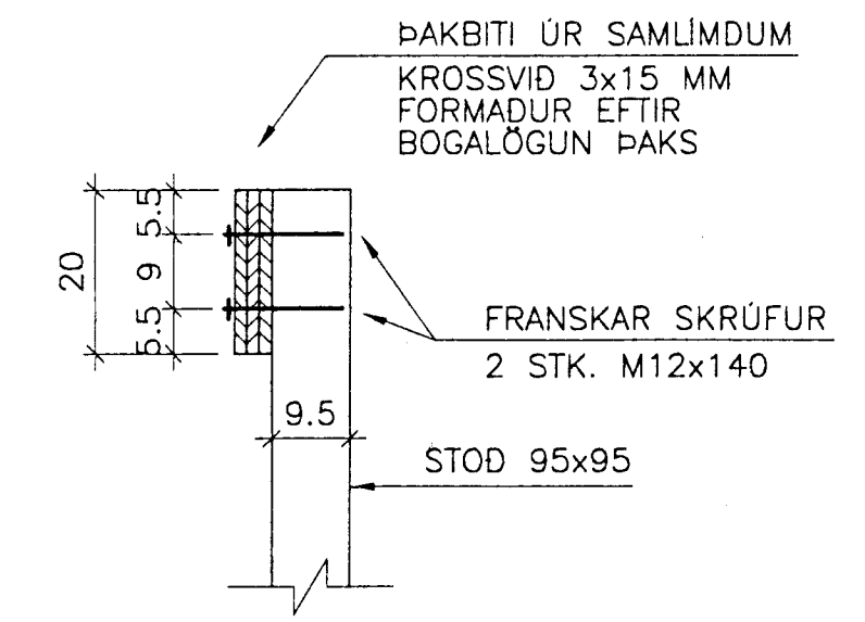
SNID G-G 1:10
