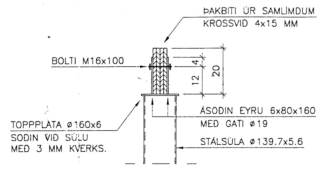
SNID E-E 1:10
