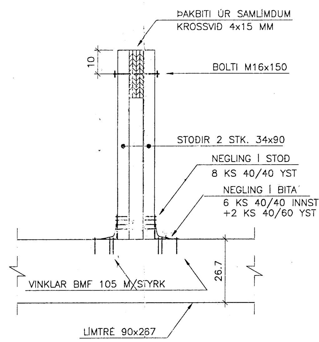
SNID F-F 1:10
