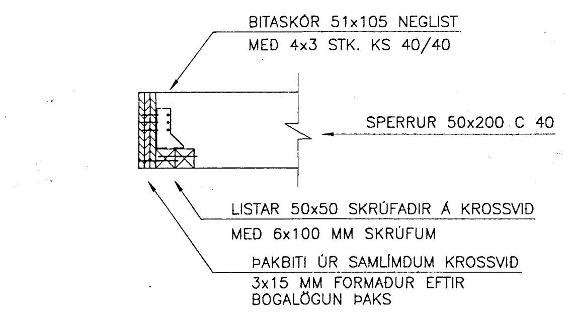
SNID H-H 1:10
