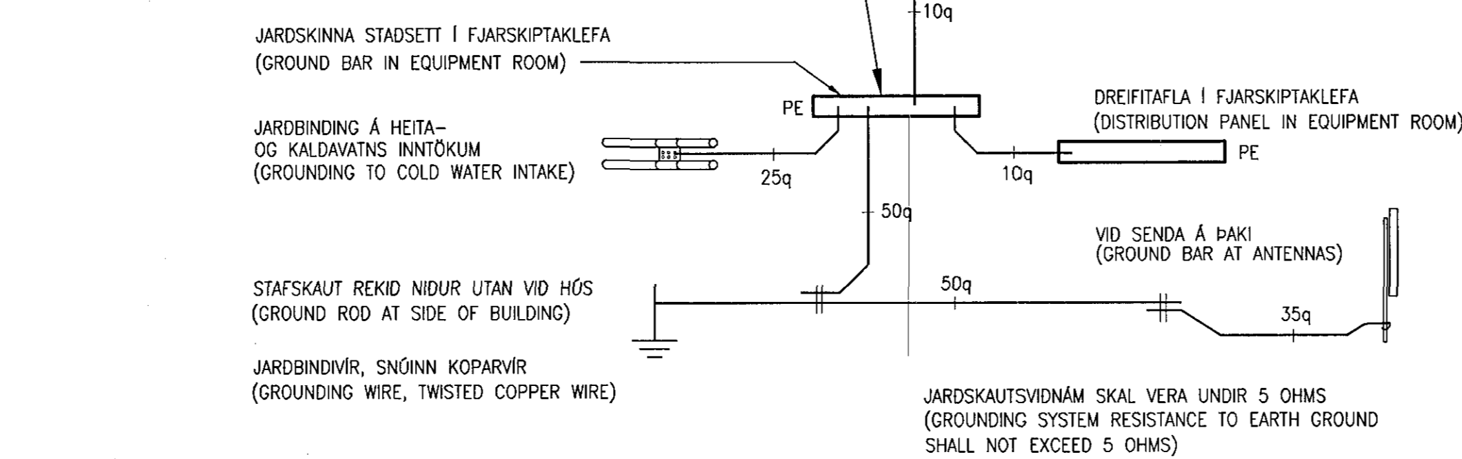
JARDTENING (GROUNDING)
