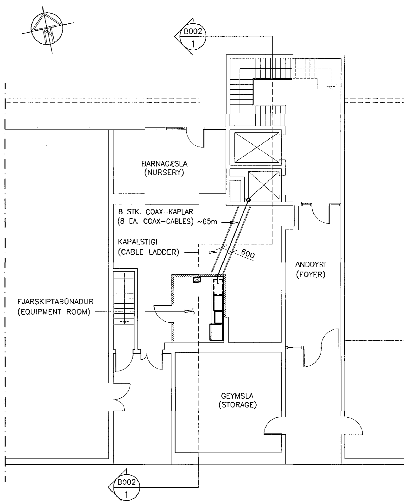
GRUNNMYND, 1.HÆÐ MKV 1:100 (1ST FLOOR PLAN SCALE 1:100)
