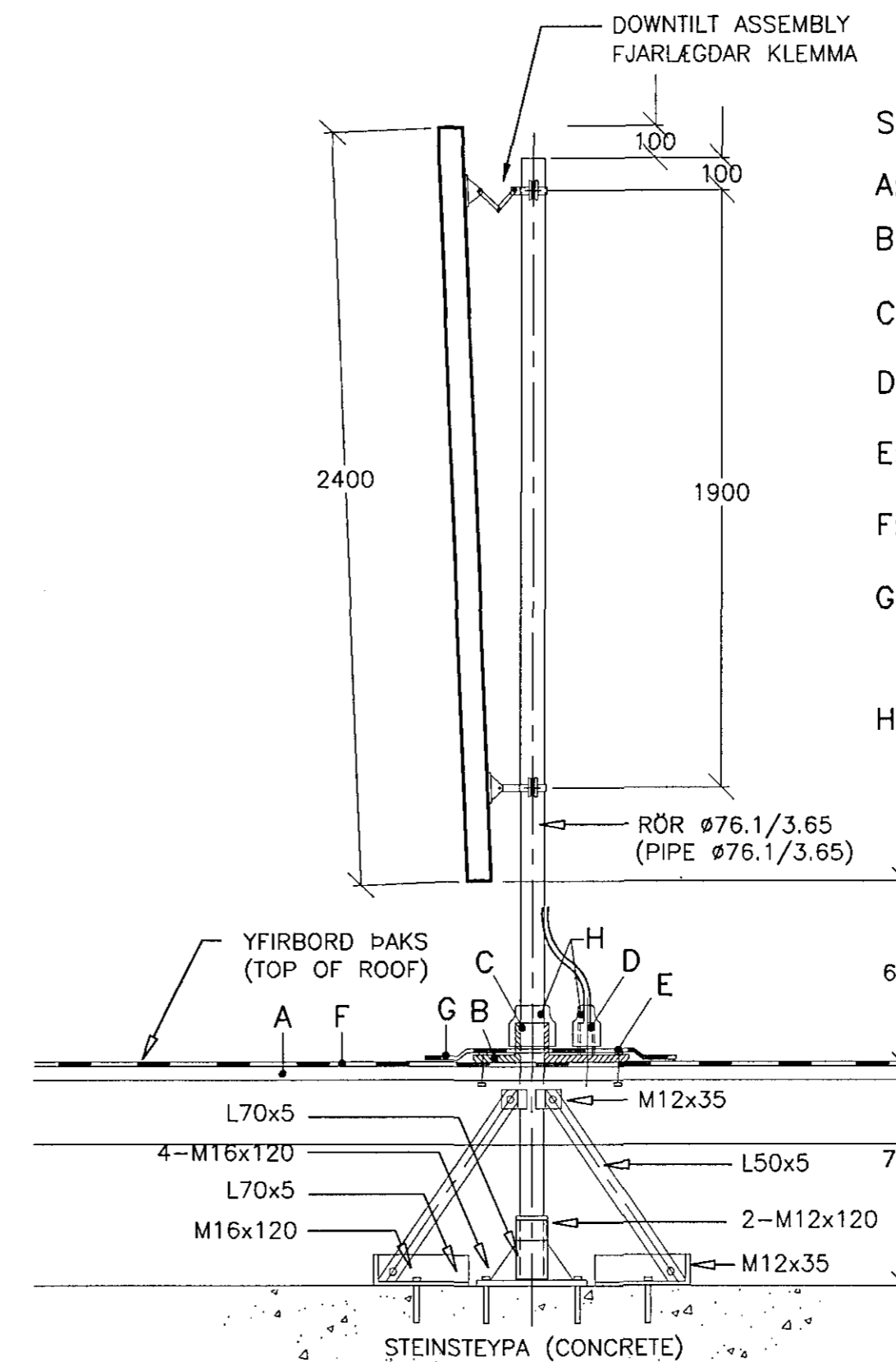
LOFTNETSFESTINGAR Á ÞAKI MKV 1:20 (ANTENNA SUPPORT ON ROOF SCALE 1:20)
