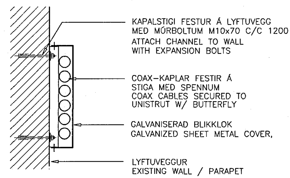
KAPALSTIGI Í LYFTUSTOKK MKV 1:10 (CABLE LADDER IN LIFT SHAFT SCALE 1:10)
