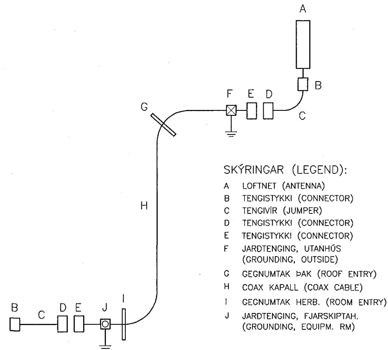
COAX KAPALL, EINLÍNEMYND (COAX CABLE, ONE LINE DIAGRAM)
