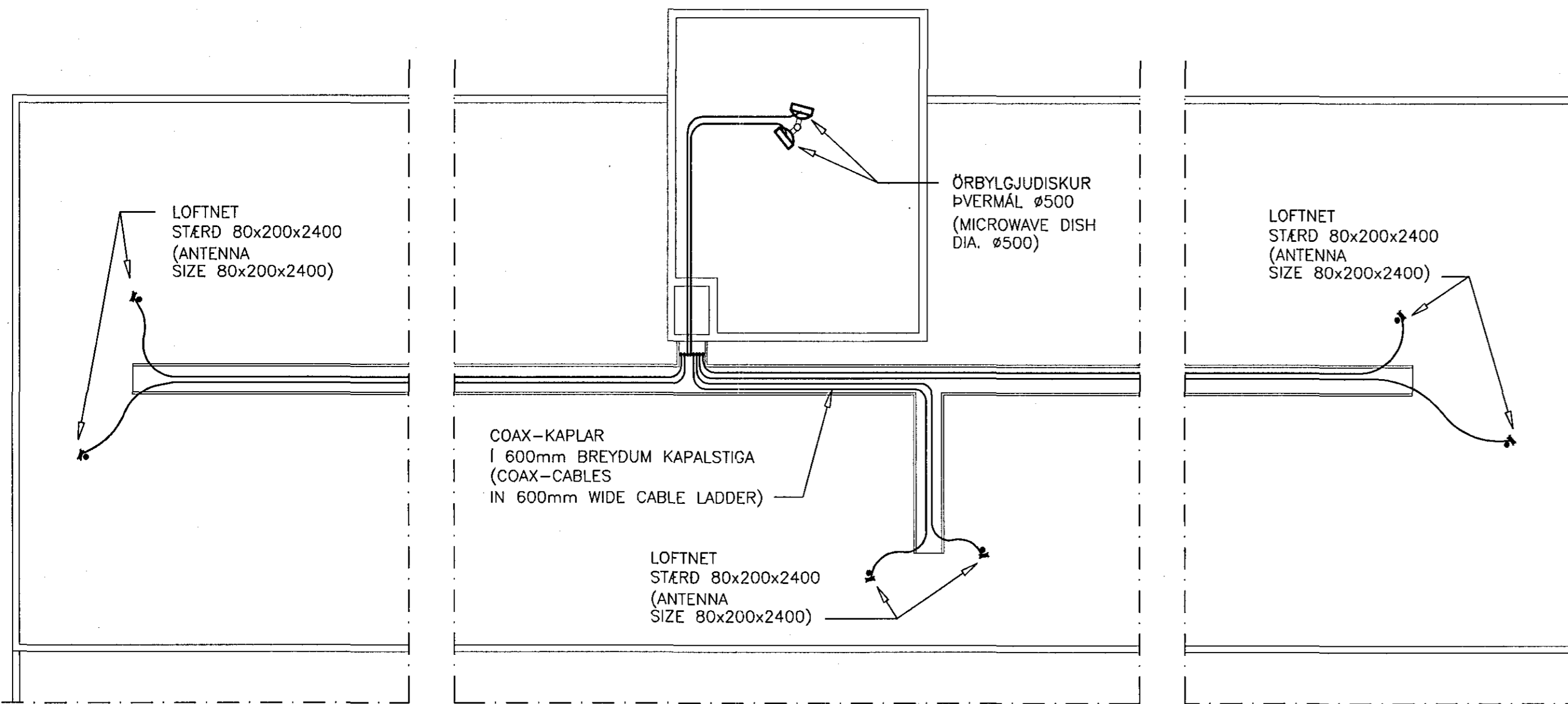
ÞAKMYND, COAX-KAPLAR MKV 1:100 (ROOF PLAN, COAX CABLES SCALE 1:100)
