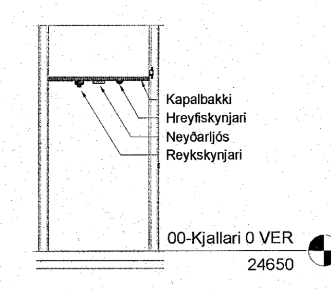
EB Snið EB 00_3_14_01 1 : 50
