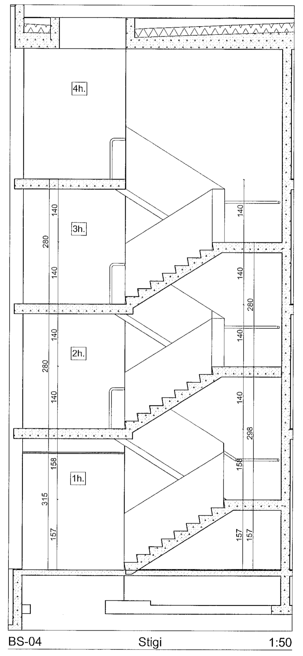
D-06 Stigabrep 1:5
