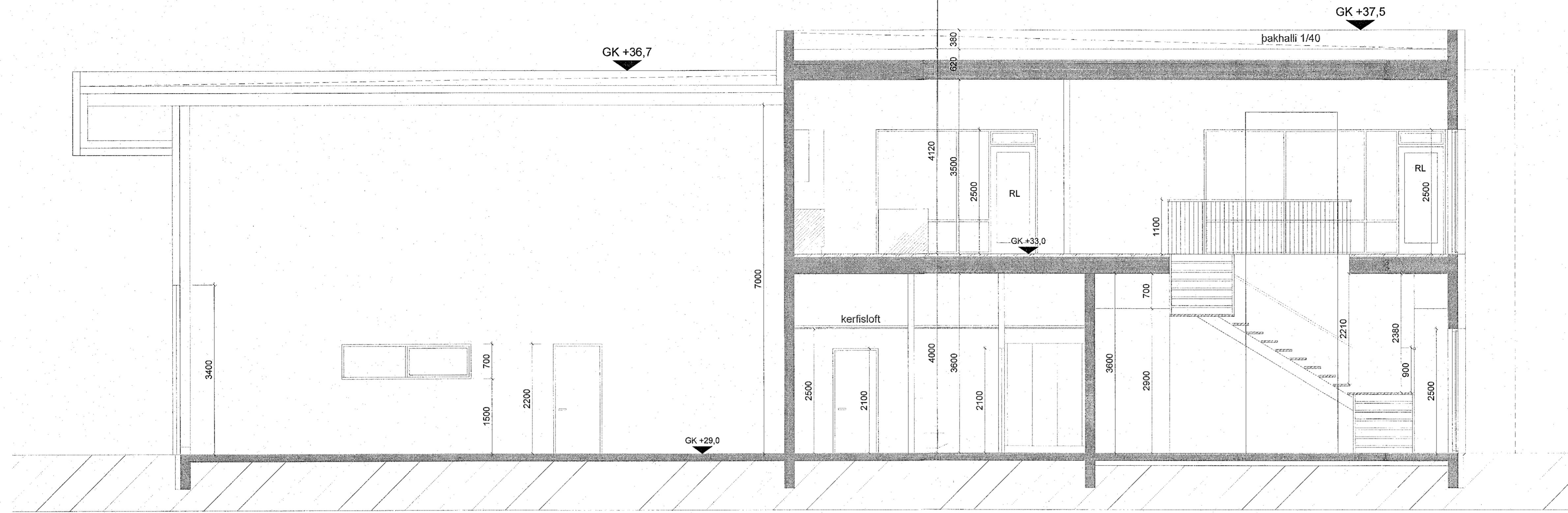
SNEIDING Y-Y 1:50
