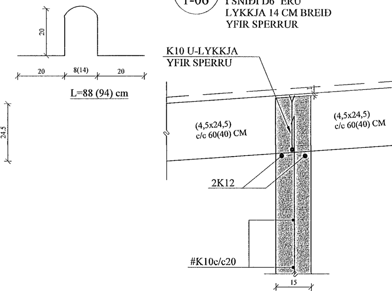
D6 SNID. 1:10 1-06
