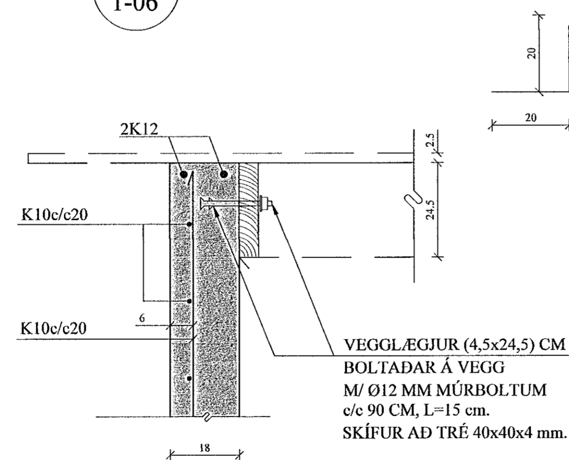
B6 SNID. 1:10 1-06
