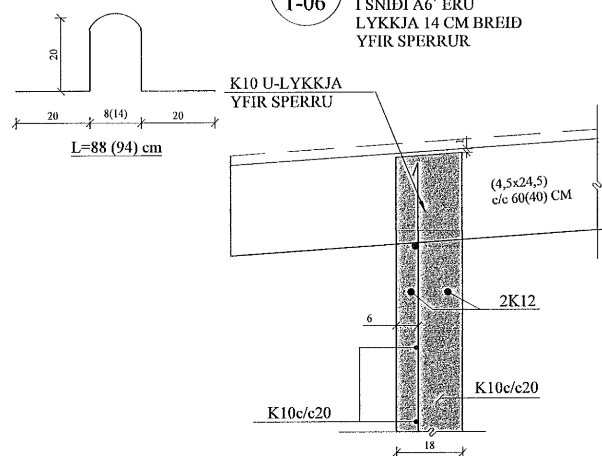
A6 SNID. 1:10 1-06
