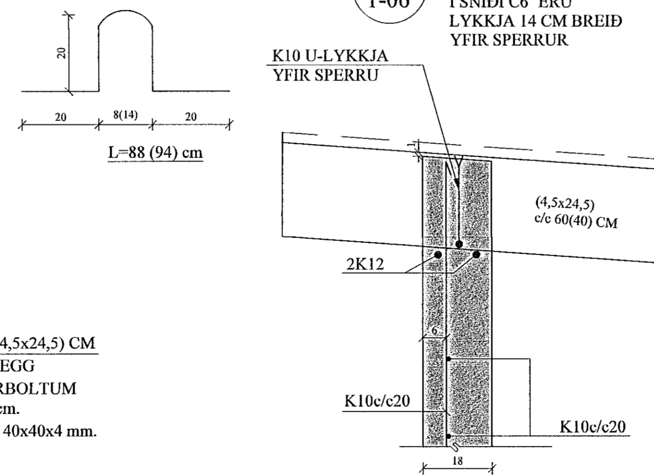
C6 SNID. 1:10 1-06
