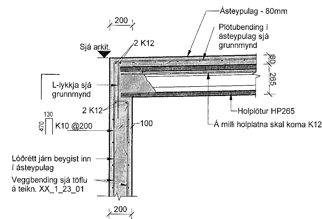
EB Snið EB 01.121.01 1 : 20
