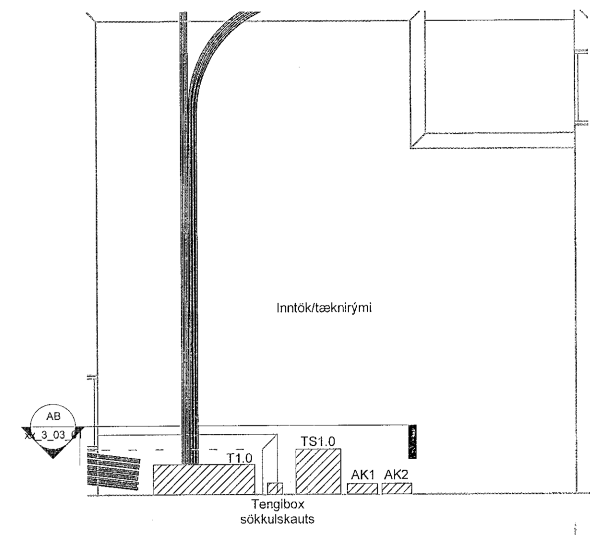
AA xx_3_03 - Deili AA xx_3_03_01 1:50
