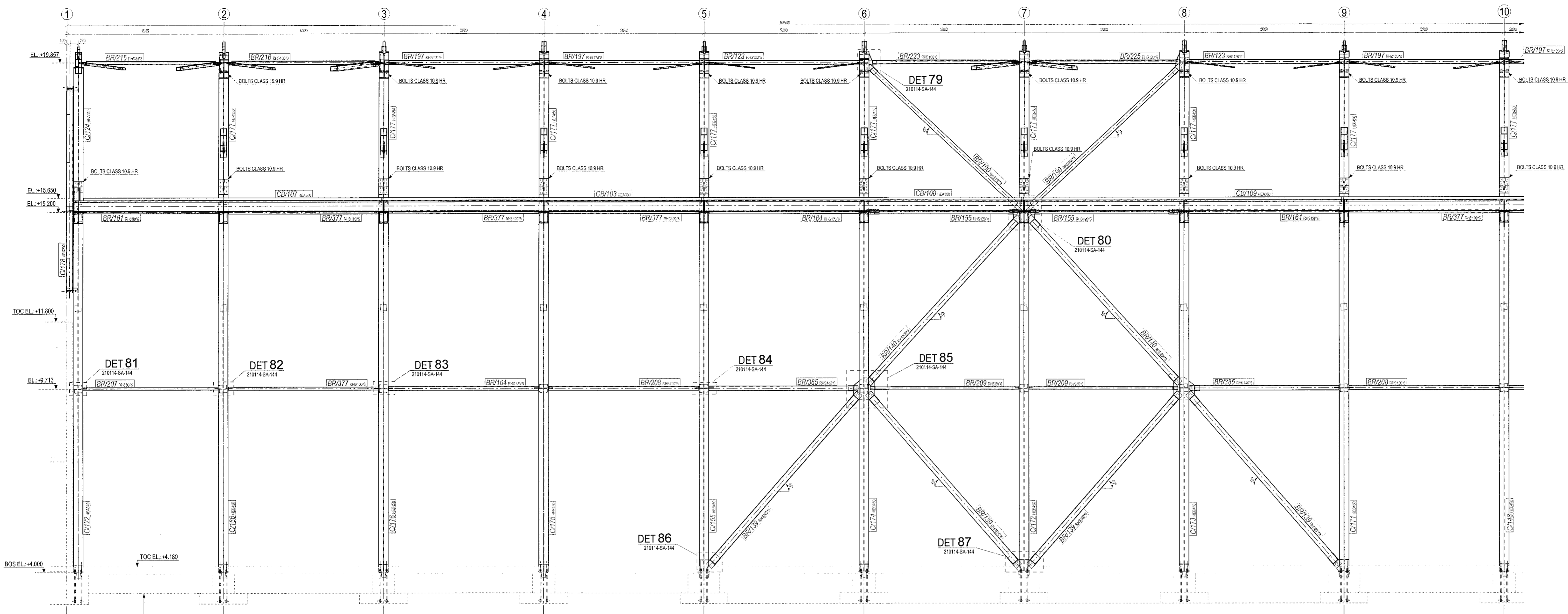
LINE B.1 - PART 1 1:50
