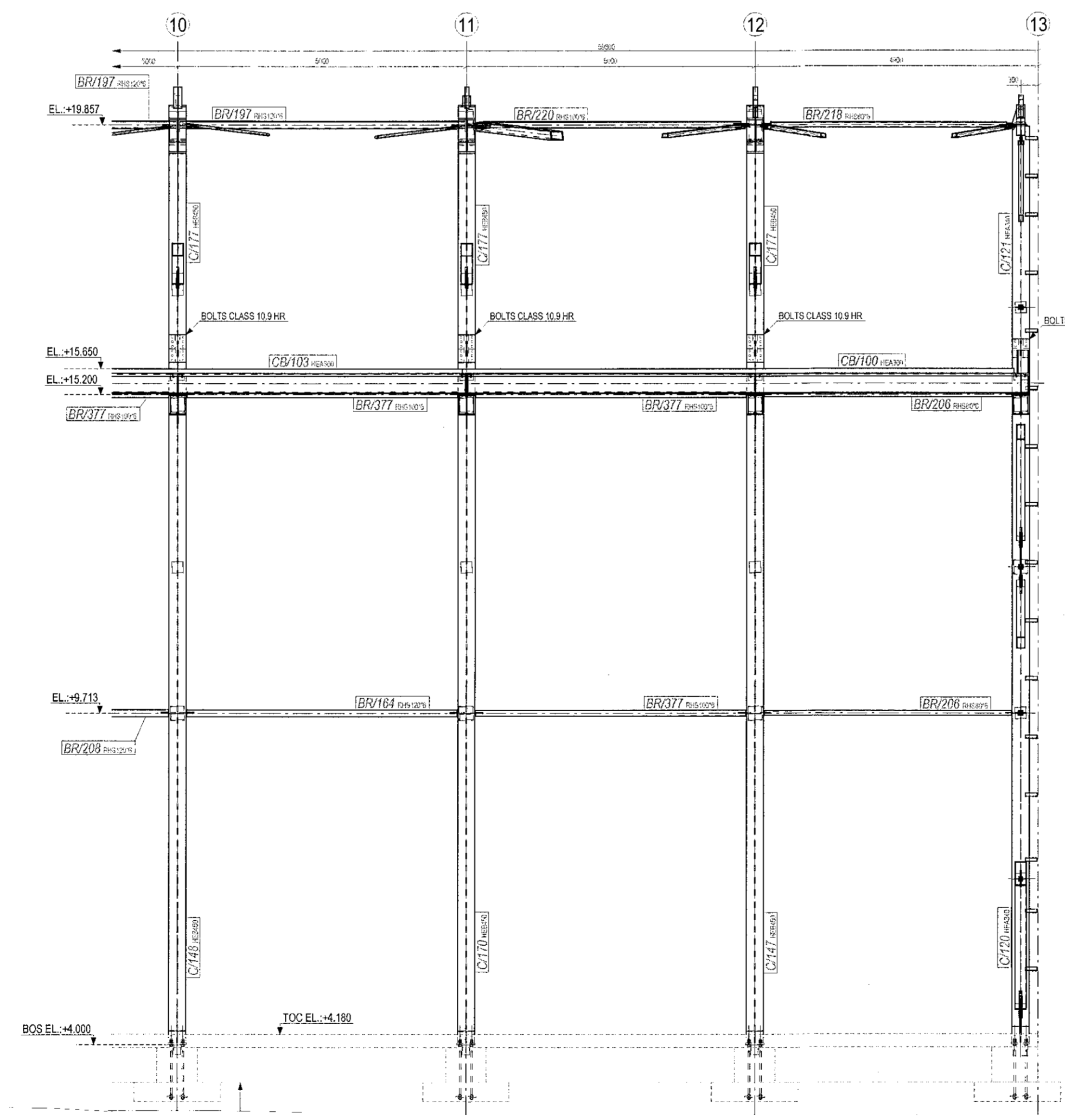
LINE B.1 - PART 2 1:50
