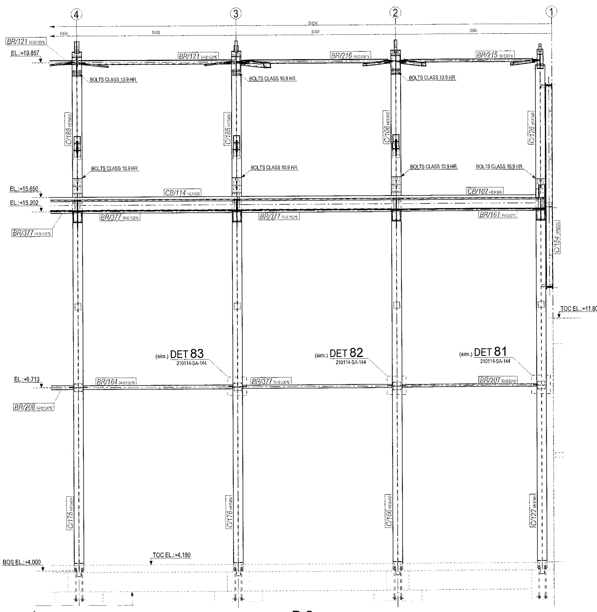
LINE B.2 - PART 2 1:50
