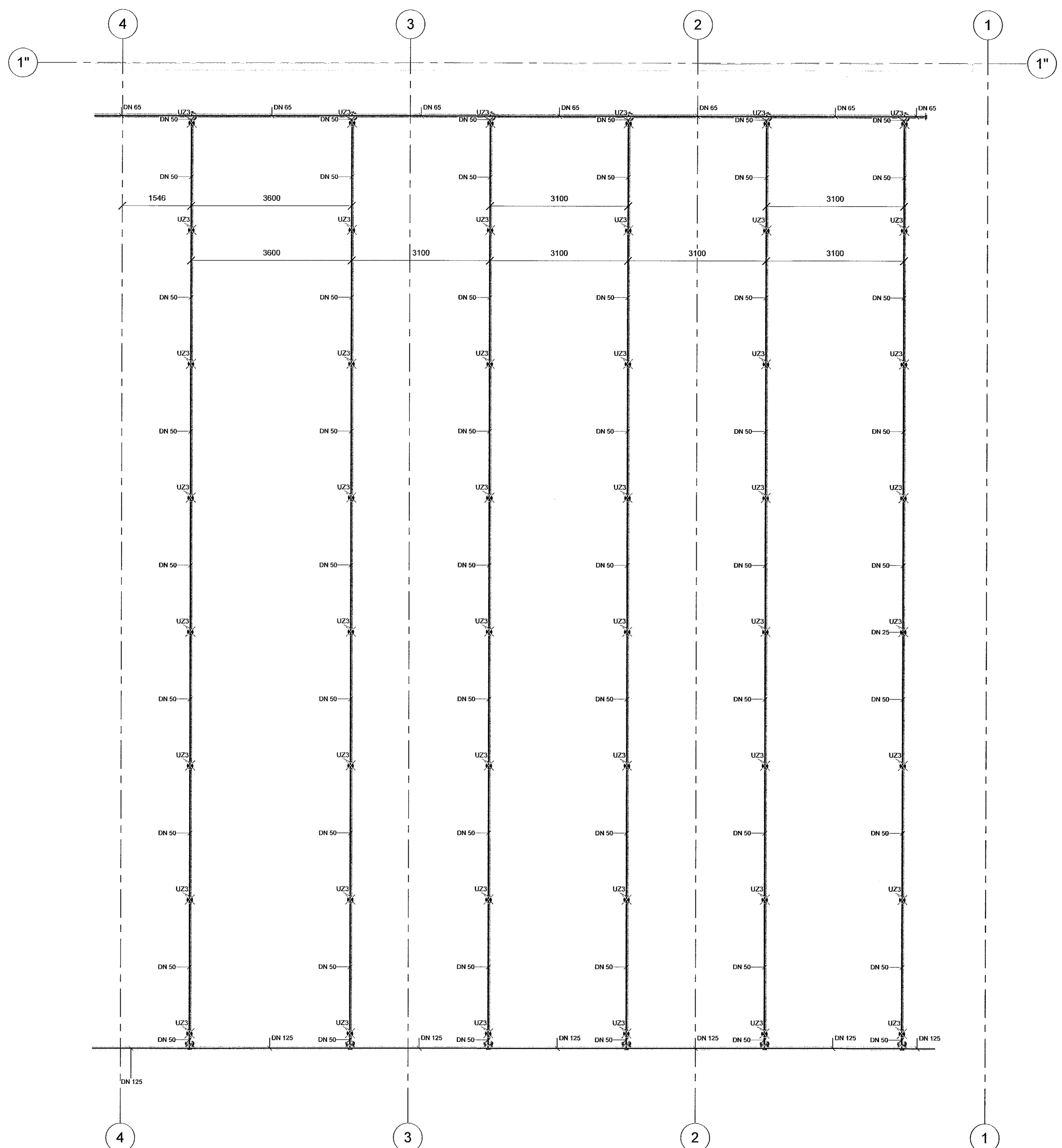
1 Lager hluti 2 1 : 50
