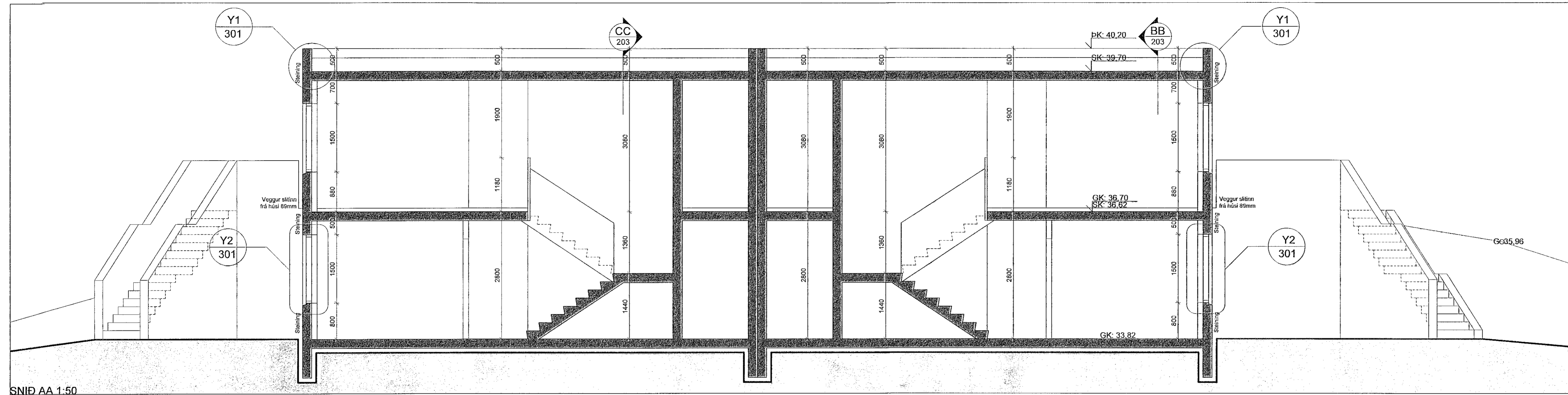
SNID AA 1:50
