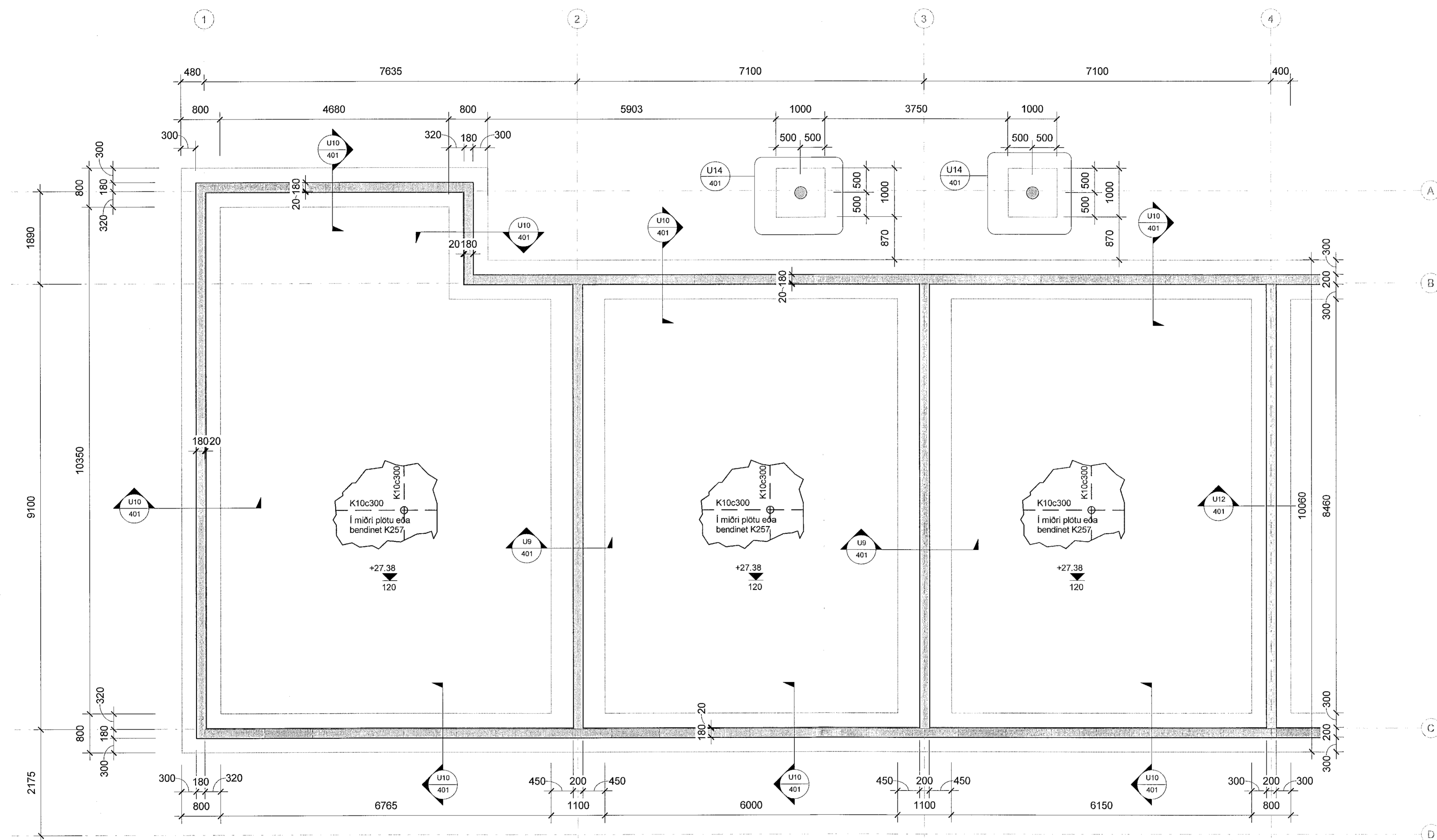
1 00 Undirstöður - 1/2 1 : 50
