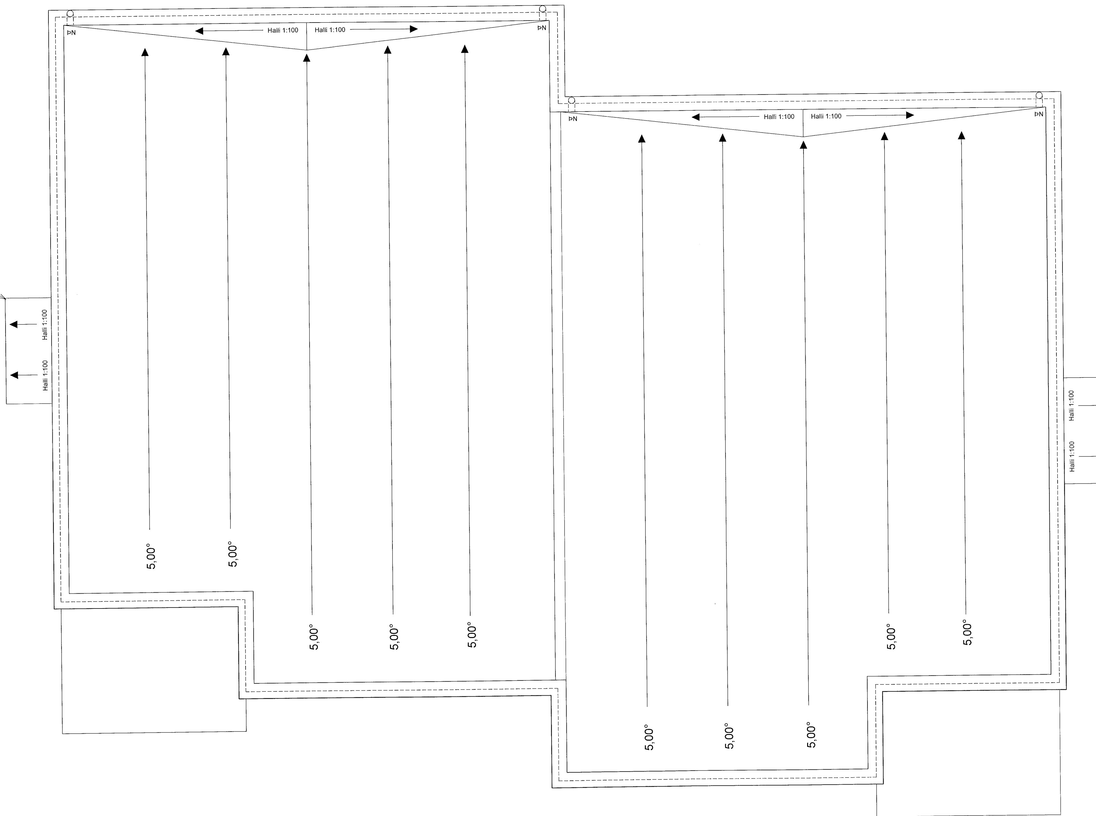
Þakhallaplan mkv: 1 : 50
