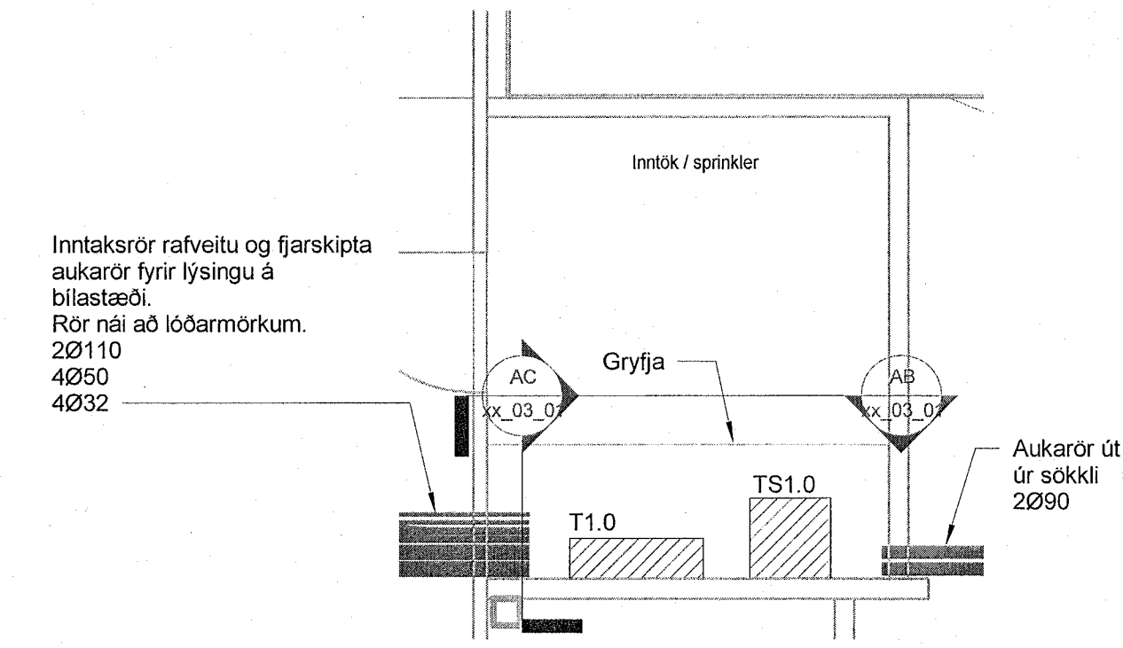
AA xx_03_01 - Deili AA xx_03_01 1:50
