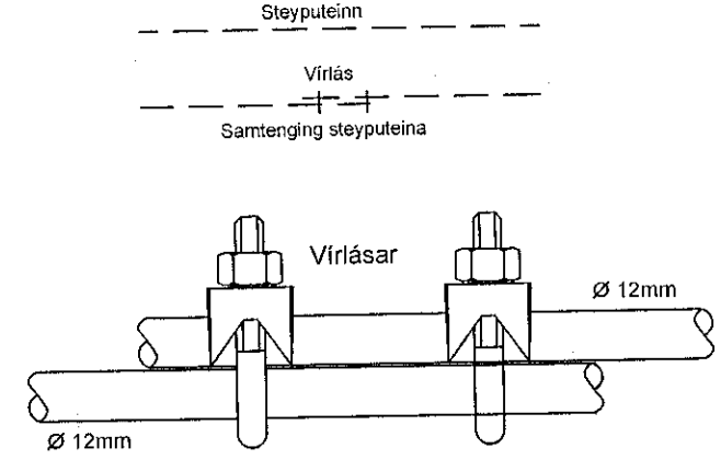
Samtenging steyputeina
