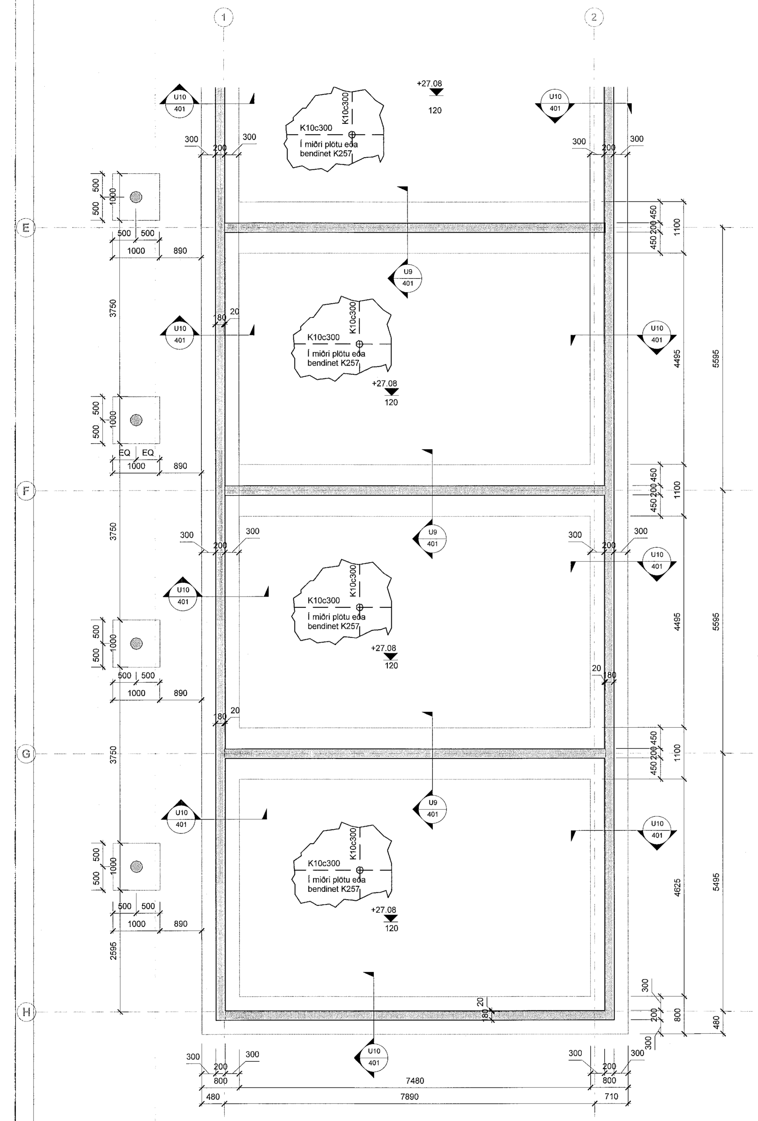
1 00 Undirstöður - 3/3 1 : 50
