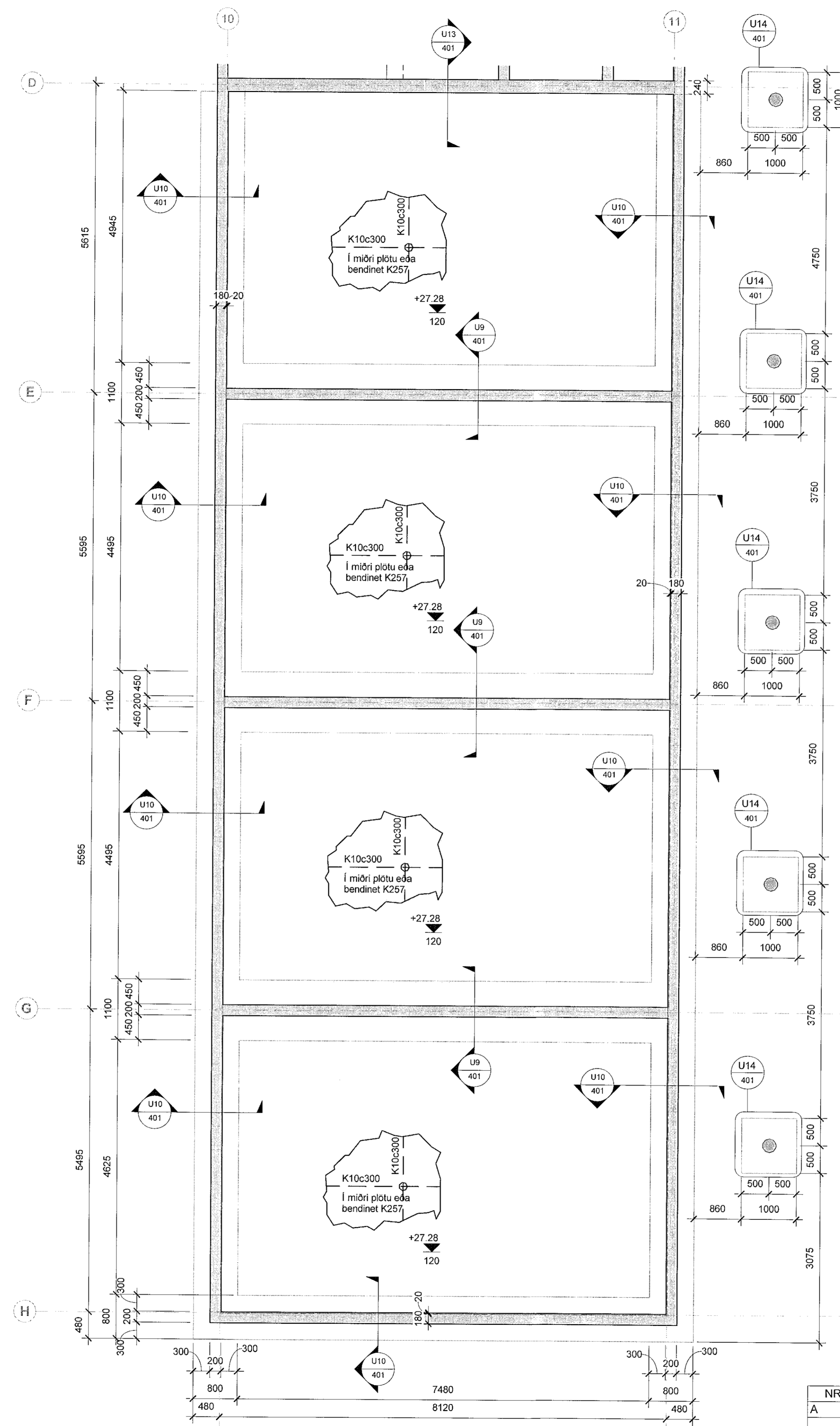
1 00 Undirstöður - 1/2 1 : 50
