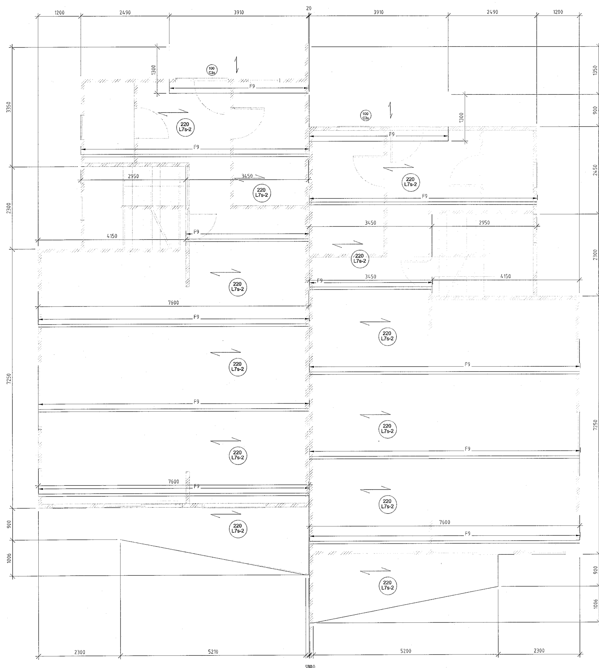
FLOOR 1:50
