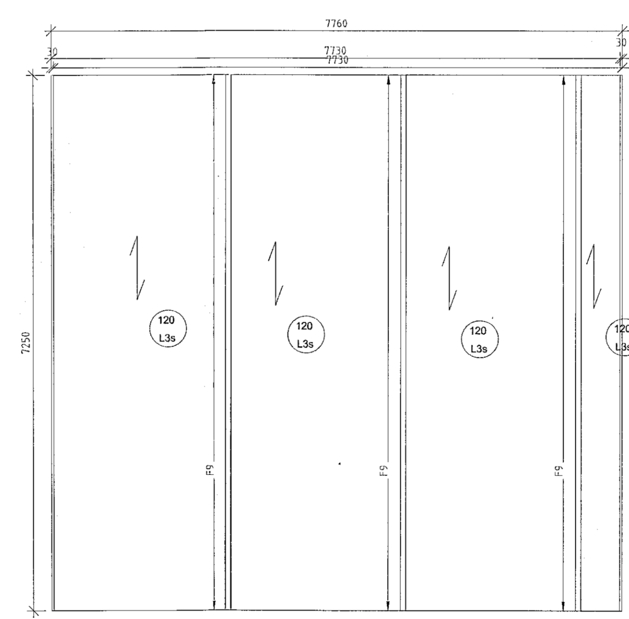
ROOF1:50
